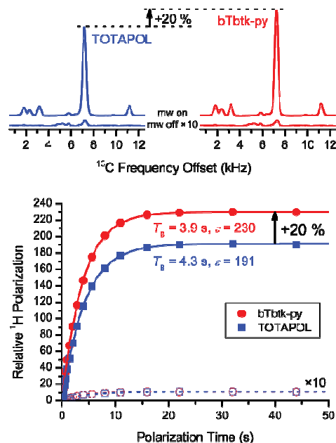
Figure 1. DNP enhanced polarization was measured under microwave irradiation using a gyrotron beam current of 34 mA, which corresponds to \sim 12 W microwave power. (Upper) 13 C-NMR (CPMAS) of 1M urea- 13 C in 60/30/10 glycerol-d 8 /D 2 O/H 2 O (v/v/v) with 10 mM of the appropriate biradical acquired with and without microwave irradiation. (Lower) Build-up curves were recorded at the respective field yielding the maximum enhancement for each radical (i.e. 4.982 T for bTbtk-py, 4.980 T for TOTAPOL; see Figure 3) and subsequently scaled in order to normalize the off signal intensities at t = \infty . Proton longitudinal relaxation time constants were determined as T_{11} = 3.9 s for bTbtk-py and T_{11} = 4.5 s for TOTAPOL. Note that aside from the radical used and the magnetic field strength, the experimental conditions are the same for each trace.
