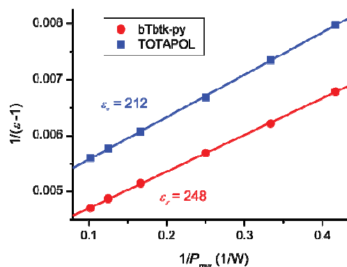
Figure 2. Power dependence of the steady-state DNP enhancement \epsilon_{\infty} for bTbtk-py and TOTAPOL given by: 1/\epsilon = 1/\epsilon_{\infty}(1+1/aP) . The experiments with the two polarizing agents were carried out at the field position giving the optimum enhancement for each. Otherwise, the experimental conditions were identical (see supporting information).
