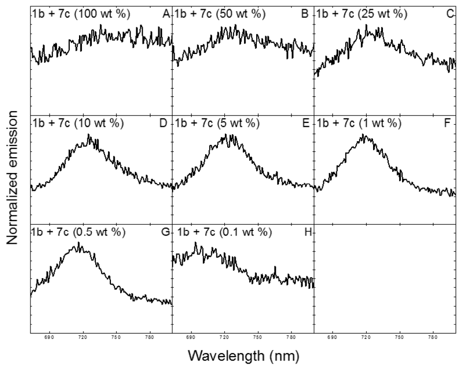
Figure S10: Thin films of polymer 1b and fluorophore 7c at various fluorophore concentrations.
