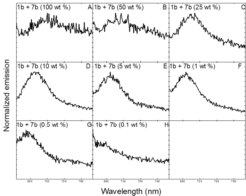
Figure S9: Thin films of polymer 1b and fluorophore 7b at various fluorophore concentrations.
