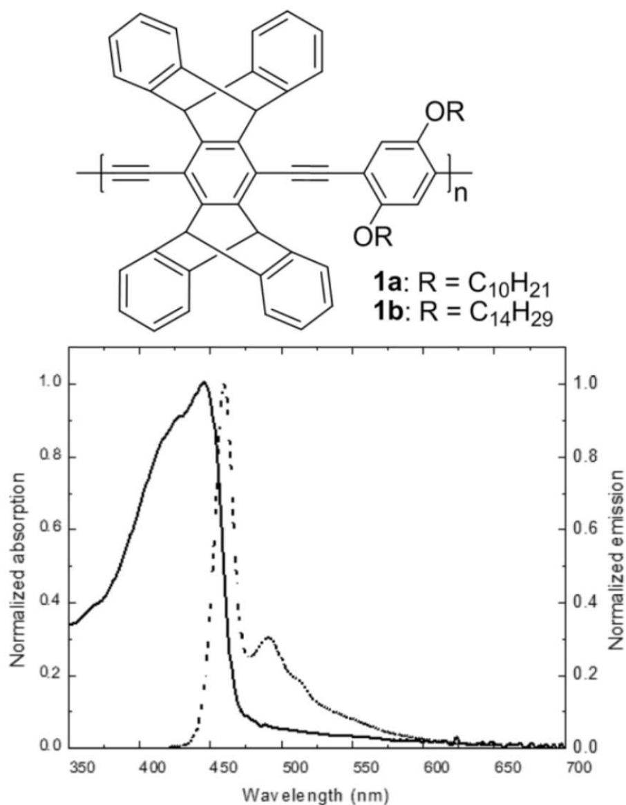
Figure 1. The absorption (solid line) and emission (dashed line) spectra of polymer 1a in spin-cast films (Thin films: \lambda_{\text{max abs.}} = 446 nm, \lambda_{\text{max em.}} = 460 nm, \Phi\text{F} = 0.33, n (633 nm) = 1.66; chloroform solution: \lambda_{\text{max abs.}} = 427 nm, \lambda_{\text{max em.}} = 453 nm, \Phi\text{F} = 0.50).
