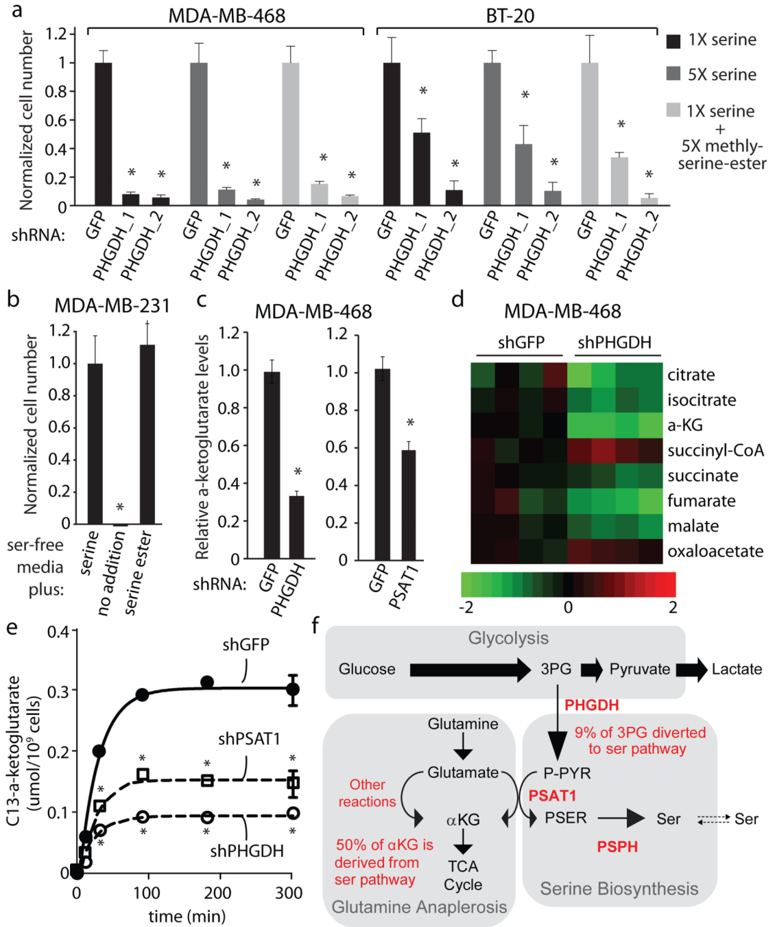
Figure 4. Suppression of PHGDH results a deficiency in anaplerosis of glutamine to alpha-ketoglutarate
