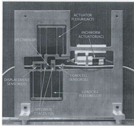
Fig. 6. Small scale tension testing machine [8].
