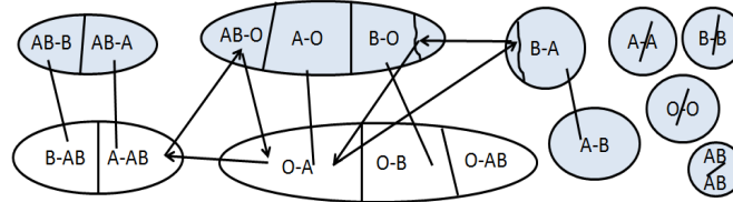
Figure 1: The structure of an efficient allocation without altruistic donors. All B-A pairs are matched to A-B (assuming more B-As than A-Bs), the remainder of the A-B pairs are matched in 3-way exchanges using O-A's and B-O's. AB-O are matched in 3-ways each using two overdemanded pairs, and every other overdemanded pair is matched to an underdemanded pair.
