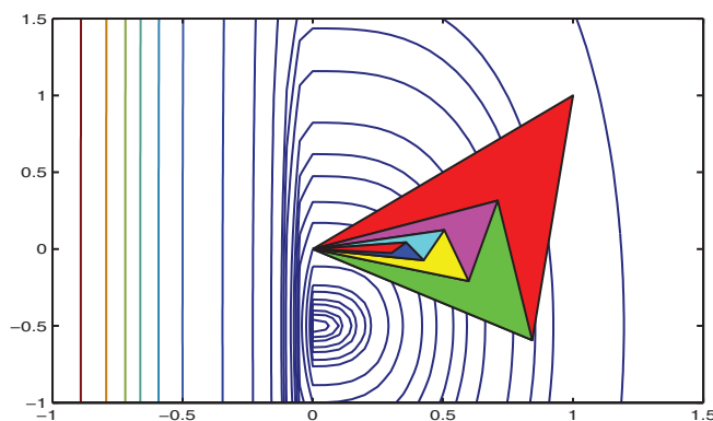
FIG. 1. The NM algorithm's failure on the McKinnon counterexample (1.1).
