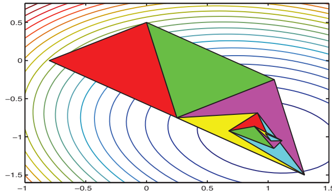
FIG. 9. Convergence of the RNM algorithm on a strictly convex quadratic function.
