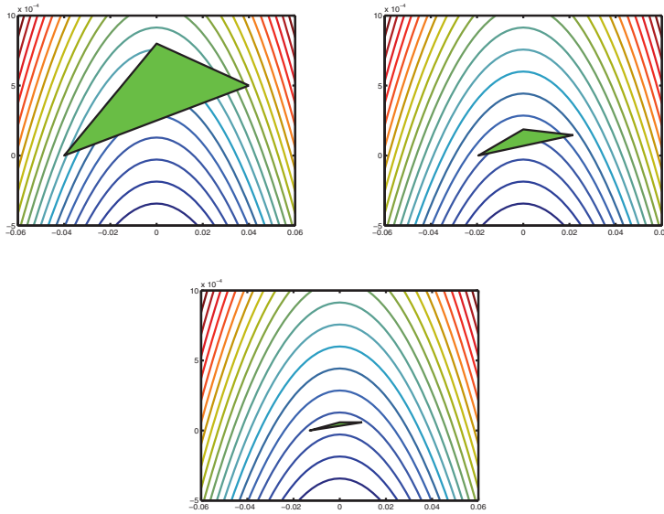
FIG. 3. Three (nonconsecutive) increasingly small, increasingly flat RNM triangles are represented, along with contours of \tilde{y} + \frac{1}{2}\tilde{x}^2 , in a neighborhood of the origin. (Note the expanded scale on the y axis.) Moving from left to right, the flatnesses are 0.043, 0.035, and 0.024.
