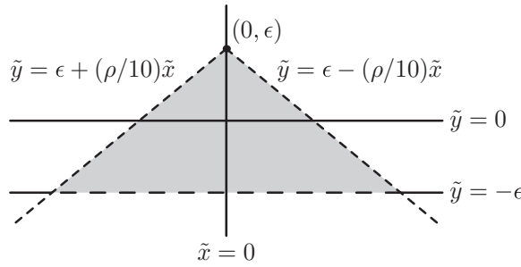
FIG. 5. The downward-pointing sector lies between the two finely dashed lines. The truncated sector (3.16) consists of the shaded area for \rho = 8 and \epsilon = 0.5 .
