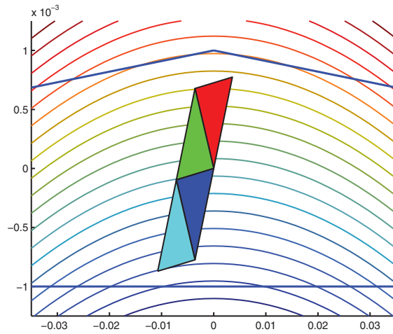
FIG. 6. The blue straight lines bound the truncated sector (3.16) for \rho = 0.09 and \epsilon = 0.001 . (Note the expanded scale on the \tilde{y} axis.) An initial RNM triangle inside the sector, with a vertex at the origin, is shown for which \tilde{h}/\tilde{w} > \rho ; contours of the surrogate function \tilde{y} + \frac{1}{2}\tilde{x}^2 , treated as the objective, are also shown. It is easy to see that the three subsequent RNM moves are reflections and that, as long as the RNM triangle remains in the sector, it will continue to reflect downward until exiting at the bottom of the sector.
