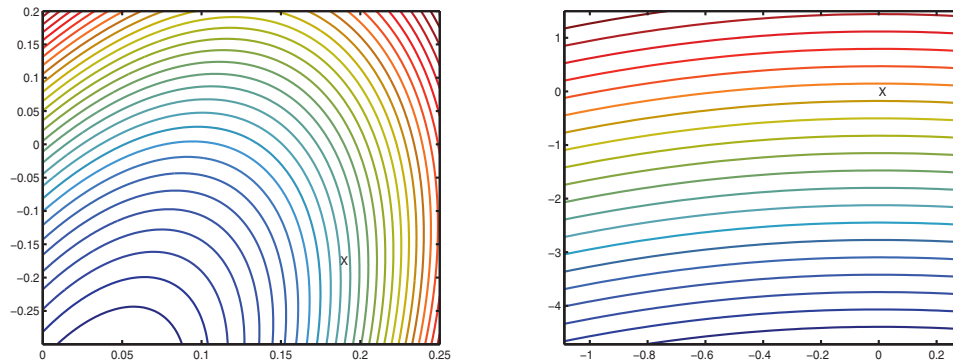
FIG. 4. The contours of -6x - y + 30x^2 + y^2 - 10xy + 2(y+1)^2 \exp(x^2) are shown on the left, in the region 0 \leq x \leq 0.25 , -0.3 \leq y \leq 0.2 . After applying the affine transformation defined in Lemma 3.1, where the base point \mathbf{b} = (0.1875, -0.15)^T is marked with an X , the contours of \tilde{y} + \frac{1}{2}\tilde{x}^2 are shown on the right in transformed coordinates (\tilde{x}, \tilde{y}) . Note that the transformed base point is the origin.
