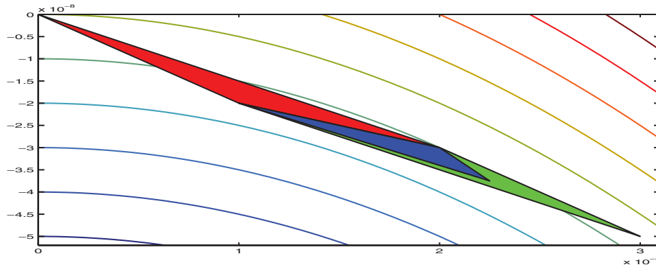
FIG. 8. The contours of \tilde{y} + \frac{1}{2}\tilde{x}^2 + \frac{1}{2}\tilde{y}^2 , are shown along with an RNM triangle with \tilde{h}/\tilde{w}^2 = \frac{3}{4} . The reflection step is not accepted, and an outside contraction is performed. Note the difference, by four orders of magnitude, between the horizontal and vertical scales.
