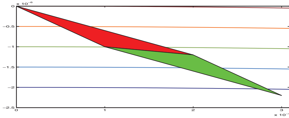
FIG. 7. The contours of \tilde{y} + \frac{1}{2}\tilde{x}^2 + \frac{1}{2}\tilde{y}^2 are shown along with an RNM triangle with \tilde{h}/\tilde{w}^2 = 30 . The reflection is accepted.
