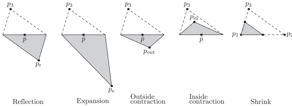
FIG. 2. The five possible moves in the original NM algorithm in two dimensions. The original simplex is surrounded by a dashed line, and its worst vertex is labeled \mathbf{p}_3 . The point \bar{\mathbf{p}} is the average of the two best vertices. The shaded figures are NM simplices following reflection, expansion, outside contraction, inside contraction, and shrink, respectively. (In the “shrink” figure, the best vertex is labeled \mathbf{p}_1 .) The “expansion” step is omitted in the RNM algorithm.
