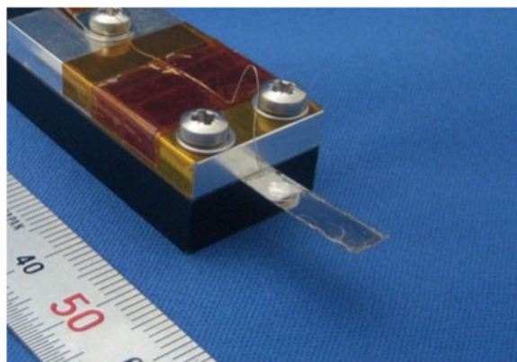
Figure 5. Fabrication flow and photograph of transferring epitaxial lead zirconate titanate (PZT) thin films to a stainless steel cantilever: 13 (step 1) deposition of c -axis oriented PZT thin films on Pt/MgO; (step 2) deposition of Cr top electrode; (step 3) bonding the PZT thin films to a stainless steel cantilever; and (step 4) etching out the MgO substrate.
