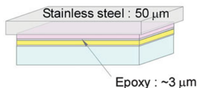
(3) Bonding with stainless steel sheet
