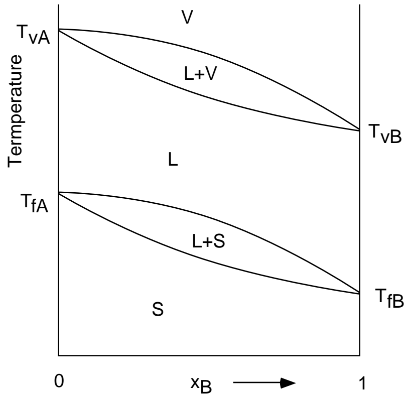
Figure 1 • Binary Phase Diagram. A binary phase diagram is an isobaric temperature-composition diagram. In this case there is complete solubility in the solid, liquid, and vapor states of aggregation, and only one phase is found for each state of aggregation. At low temperatures, the material of any composition is solid; at higher temperatures there is a two-phase liquid-plus-solid region, a liquid region, a liquid-plus-vapor region and, at very high temperatures, an all-vapor region.
