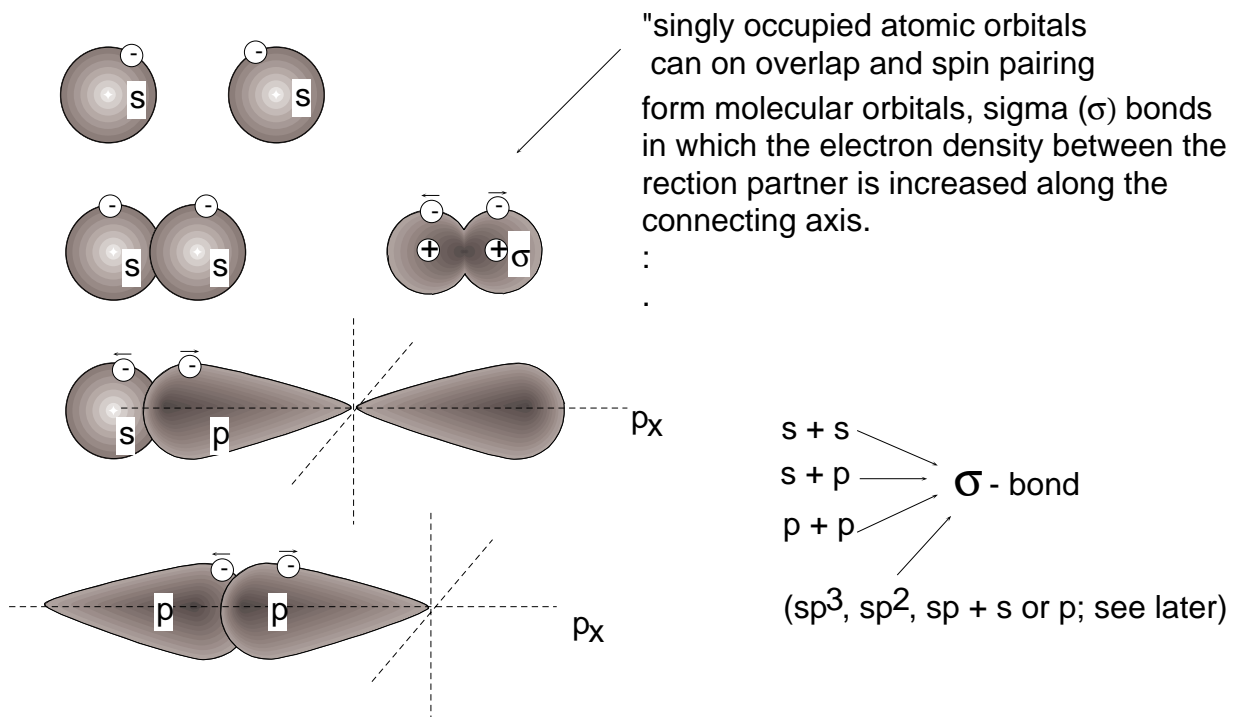
Figure 5 Covalent bond formation
