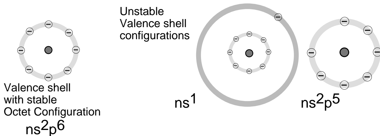
Fig.1 Stable and Unstable Valence Shell Configurations.
