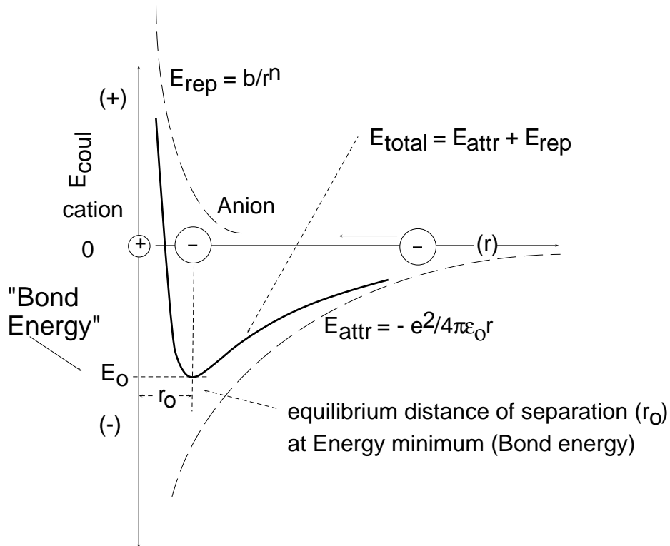
Figure 3 Energetics of ionic bonding. corresponds to the energy minimum for the NaCl molecules:
