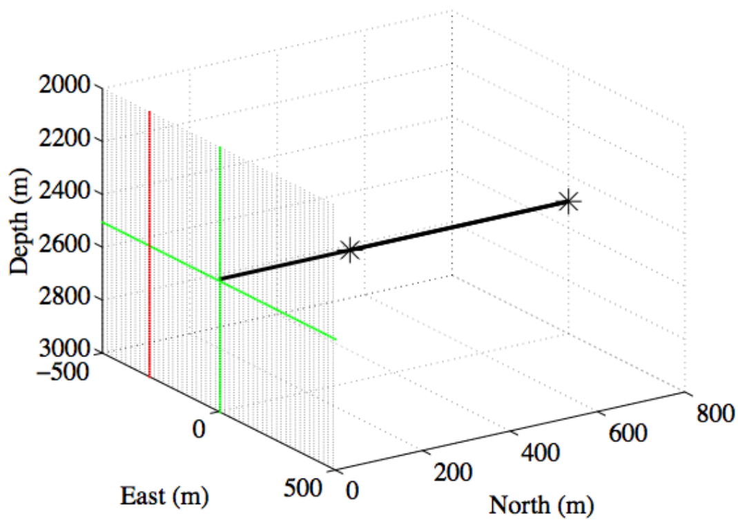
Source-receiver geometry
