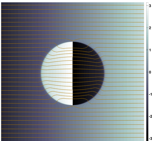
FIG. 4 (color online). The “stream lines” of the probability flux “going through” the nanoparticle. Background color depicts the phase distribution of the wave function. The 2\pi phase jump at the centerline of the nanoparticle is a numerical artifact. Here the parameters we use are a = 2 nm, a_c = 1.5 nm, m_1 = 0.9 , m_2 = 2.2 , and, correspondingly, V_1 = 0.057 eV and V_2 = -0.788 eV.
