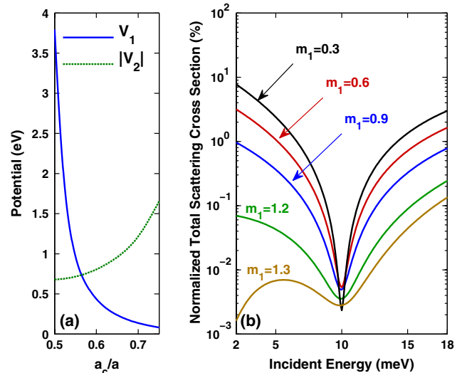
FIG. 5 (color online). (a) The potentials can be tuned in a wide range by adjusting the ratio between the radii of the core and the shell. Here m_1 = m_2 = m_0 = 1 and a = 2 nm. (b) The energy dependence of the scattering rates is highly tunable by adjusting, for example, the effective mass of the core m_1 . For this plot m_2 = 2.2 , m_0 = 1 , and a_c = 0.75a = 1.5 nm.
