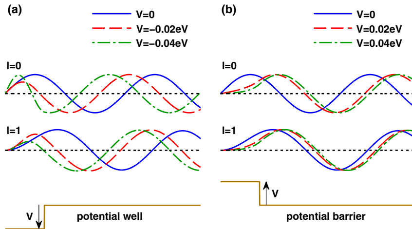
FIG. 1 (color online). Effects of potential wells and barriers on the PWs. (a) The “pulling-in” effect of a well on the 0th and 1st order PW; (b) The “pushing-out” effect of a barrier on the 0th and 1st order PW.
