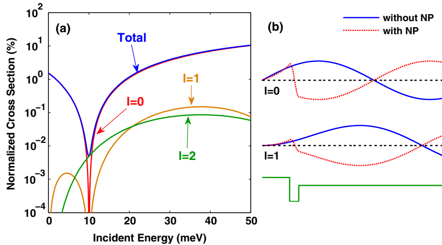
FIG. 3 (color online). (a) The total scattering cross section and the contributions from the first 3 PWs versus energy. Here the parameters we use are a = 2 nm, a_c = 1.5 nm, m_1 = 0.9 , m_2 = 2.2 , and correspondingly V_1 = 0.057 eV and V_2 = -0.788 eV. (b) The radial distribution functions of the 0th and 1st PWs with and without the nanoparticle, showing the phase shift of \pi as expected.
