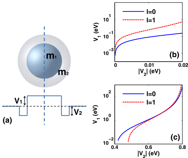
FIG. 2 (color online). (a) Conceptual illustration of the core-shell nanoparticle. V_1 is the height of the core potential and |V_2| the depth of the shell potential. (b) Combinations of V_1 and V_2 that make the phase shift of the 0th and 1st PW equal to zero, respectively. The two curves do not intersect, thus there is no common solution. (c) Combinations of V_1 and V_2 that make the phase shift of the 0th and 1st PW equal to \pi respectively. The two curves intersect at V_1 = 3.589 eV and V_2 = -0.671 eV. In this case m_1 = m_2 = m_0 = 1 , and a = 2 nm, a_c = 0.5a = 1 nm.
