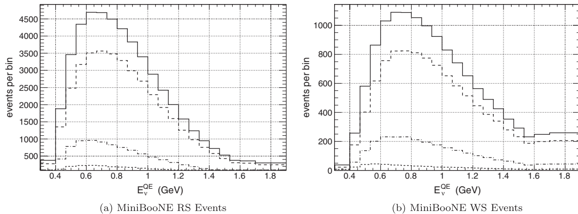
FIG. 6. Reconstructed antineutrino and neutrino energy ( E_{\nu}^{\text{QE}} ) distributions for selected RS and WS MiniBooNE events for different interaction types (CCQE, \text{CC}1\pi , other) from MiniBooNE MC. Total events are represented by the solid line, CCQE interaction events are represented by the dashed line, \text{CC}1\pi interaction events are represented by the dot-dashed line, and all other interaction (CC multi- \pi or NC) events are represented by the short-dashed line.
