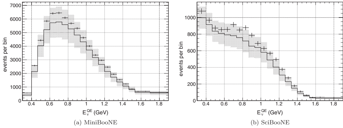
FIG. 13. Reconstructed antineutrino energy ( E_{\nu}^{QE} ) distribution for data events, compared to Monte Carlo predictions, for MiniBooNE and SciBooNE. Vertical error bars on data are statistical uncertainty. Shaded error band around simulation is the systematic uncertainty computed as the square roots of the diagonals of the total error matrix.
