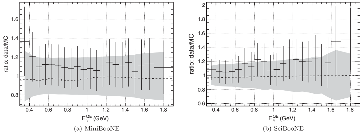
FIG. 16. The ratio, with error bars, between data and default MC as a function of reconstructed antineutrino energy ( E_{\nu}^{\text{QE}} ). The ratio of best fit signal MC to default MC is also shown (dashed line). The best fit results from the joint analysis were used to generate the signal MC. The shaded regions are the 1\sigma band from fake data with statistical and systematic fluctuations but no oscillation signal.
