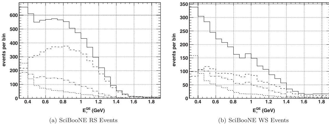
FIG. 8. Reconstructed antineutrino and neutrino energy ( E_{\nu}^{\text{QE}} ) distributions for selected RS and WS SciBooNE events for different interaction types (CCQE, CC1 \pi , other) from SciBooNE MC. Total events are represented by the solid line, CCQE interaction events are represented by the dashed line, CC1 \pi interaction events are represented by the dot-dashed line, and all other interaction (CC multi- \pi or NC) events are represented by the short-dashed line.
