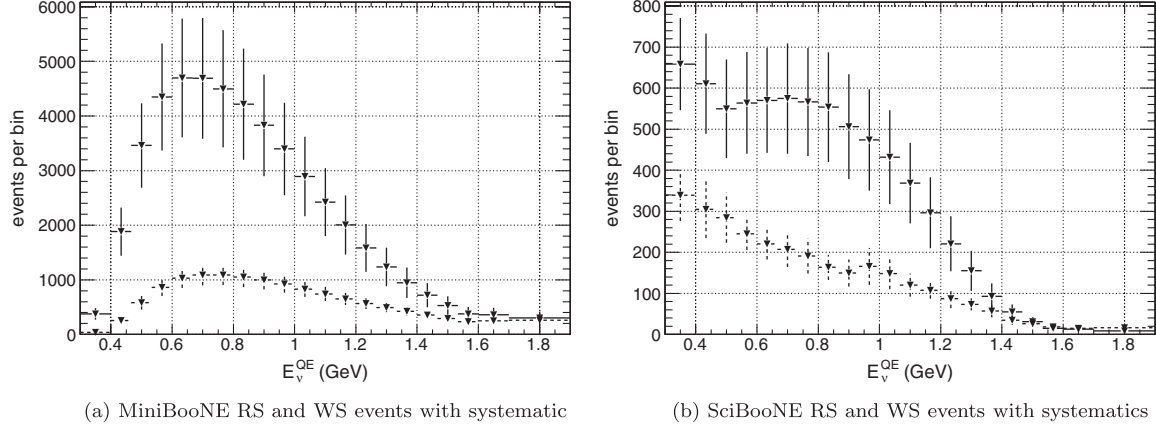
FIG. 12. RS (solid line) and WS (dashed line) contributions to the default MC prediction for MiniBooNE and SciBooNE reconstructed antineutrino and neutrino energy ( E_{\nu}^{\text{QE}} ) distributions. Error bars are the systematic uncertainties from the diagonals of the error matrix ( \sigma_{ii} = \sqrt{M_{ii}} ) and do not account for correlations.
