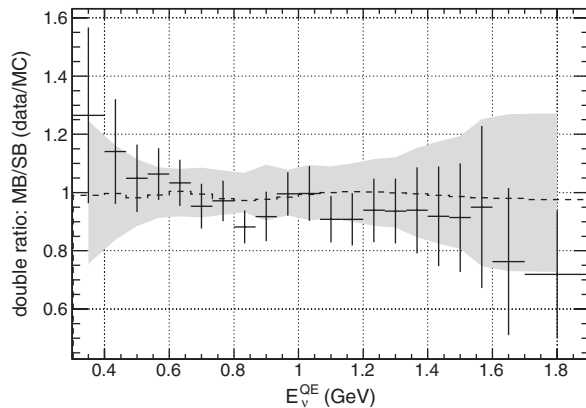
FIG. 17. The double ratio [Eq. (11)], with error bars, as a function of reconstructed antineutrino energy ( E_{\nu}^{\text{QE}} ). Some of the MiniBooNE and SciBooNE uncertainties cancel in this double ratio. The double ratio where the MiniBooNE and SciBooNE signal MC based on the best fit results from the joint analysis are used in place of data is also shown (dashed line). The shaded region is the 1\sigma band from fake data with statistical and systematic fluctuations but no oscillation signal.
