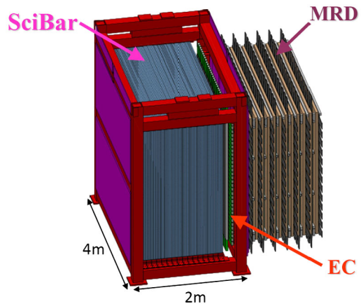
FIG. 4 (color online). Schematic view of the SciBooNE detector.
