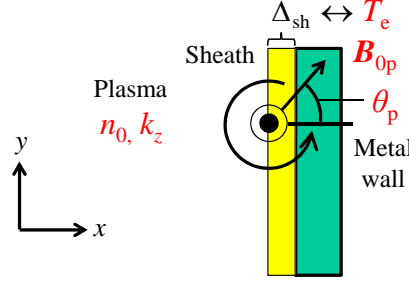
Figure 4-18: The quantities varied in the electrostatic sheath mode analysis.
