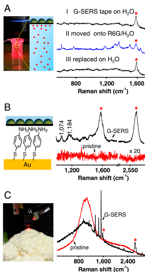
Fig. 5. Analyzing trace amounts of molecules under a variety of situations using the transparent, freestanding and flexible G-SERS(Au) substrate. (A) A real time and reversible G-SERS characterization of R6G directly in a 1 \times 10^{-5} M aqueous solution. (I, II, III are the Raman spectra with the same G-SERS tape on H 2 O, R6G/H 2 O and replaced on H 2 O, respectively). (B) Pristine (red line) and G-SERS (black line) measurements of a self-assembled monolayer of p -aminothiophenol on a flat gold surface. (C) Pristine (red line) and G-SERS (black line) measurements of a cauliflower surface with adsorbed CuPc (by soaking in a 1 \times 10^{-5} M CuPc solution in ethanol for 10 min). “*” marks the enhanced G-band and G'-band features of 1LG. Sample structures are shown in the left insets.
