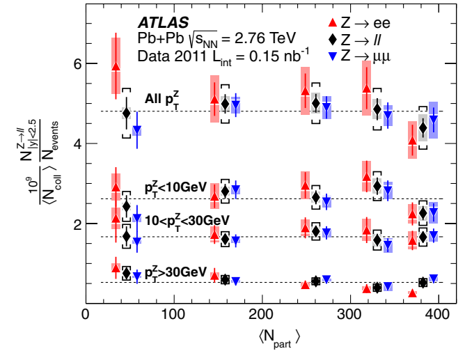
FIG. 4 (color online). Centrality dependence of Z boson yields divided by \langle N_{\text{coll}} \rangle . Results for ee (upward pointing triangles) and \mu\mu (downward pointing triangles) channels are shifted left and right, respectively, from their weighted average (diamonds). Bars and boxes represent statistical and systematic uncertainties, respectively. For the combined results, the brackets show the combined uncertainty including the uncertainty on \langle N_{\text{coll}} \rangle , and the dashed lines show the results of fits, using a constant.
