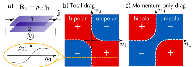
FIG. 1 (color online). Different mechanisms for Coulomb drag in graphene heterostructures. The E mechanism dominates over the P mechanism near zero doping, whereas the P mechanism dominates at higher doping. The sign of the drag response depends on carrier polarity (a). For potential fluctuations of equal sign in the two layers, Eq. (1), the net drag (b) features a pair of nodal lines (white dashed lines). Positive drag in the avoided crossing region at zero doping is dominated by the E mechanism. The resulting dependence is distinct from P -mechanism-only drag (c) smeared by correlated density fluctuations, \delta \mu_1 \approx \delta \mu_2 .
