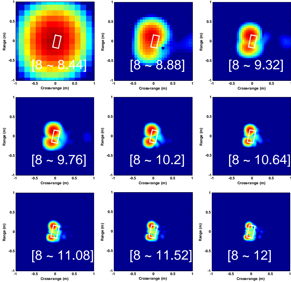
Fig. 5 Processed images of the intact specimen with various bandwidths
