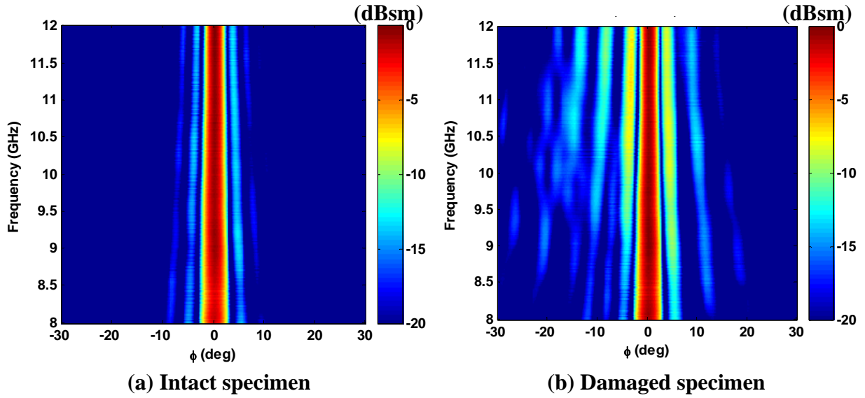
Fig. 3 Frequency-angle data of the intact and damaged specimens (HH polarization, 8GHz ~12 GHz)
