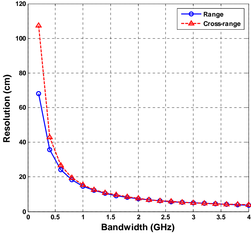
Fig. 9 Range and cross-range resolutions versus bandwidth – constant center frequency
