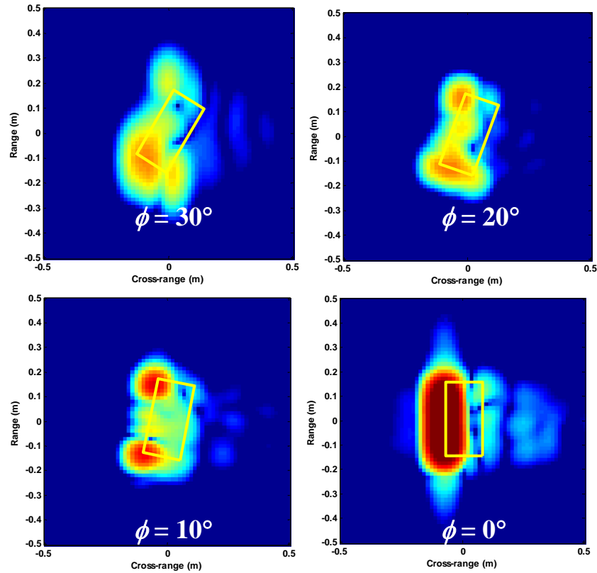
Fig. 6 Reconstructed images of the intact GFRP-concrete specimen ( \phi = 30^\circ \sim 0^\circ )
