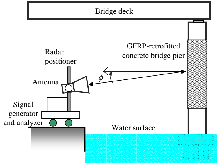
Fig. 1 Inspection scheme of the FAR NDT technique
