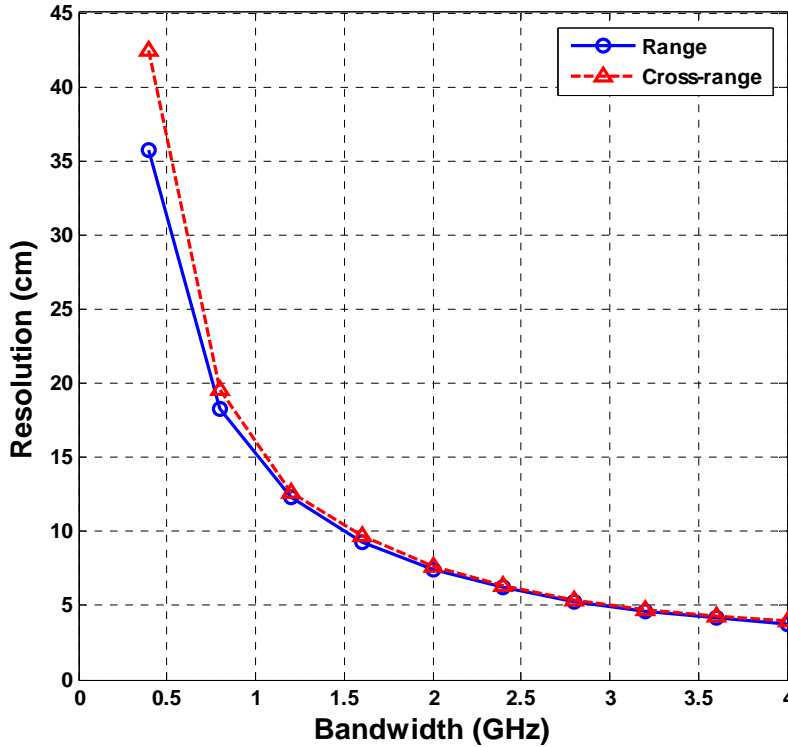
Fig. 4 Range and cross-range resolutions versus bandwidth – shifting center frequency
