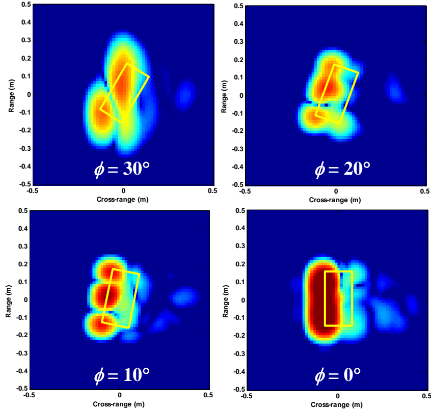
Fig. 7 Reconstructed images of the damaged GFRP-concrete specimen ( \phi = 30^\circ \sim 0^\circ )
