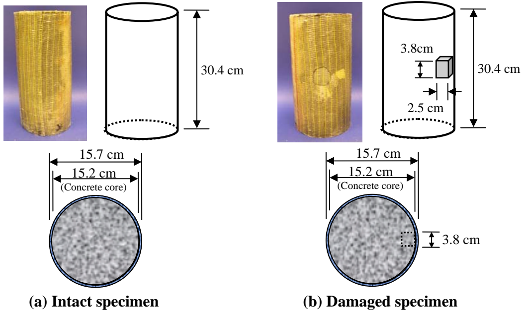
Fig. 2 Intact and damaged GFRP-wrapped concrete cylinder specimens
