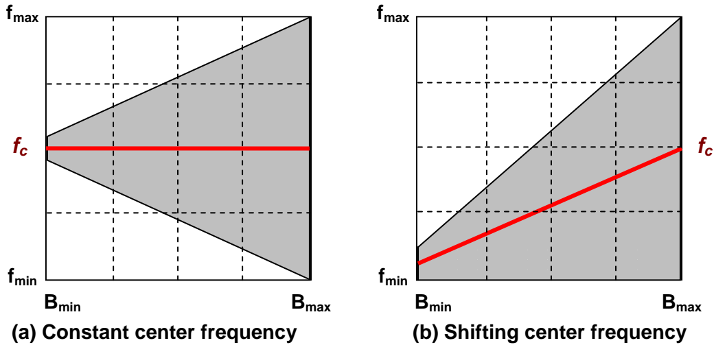
Fig. 8 Constant and shifting center frequency schemes
