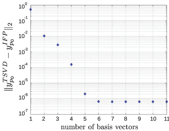
FIG. 6.9. The error in prediction outputs \|y_{p_0}^{TSVD} - y_{p_0}^{IFP}\|_2 between the TSVD and IFP predictions vs. the number of IFP basis vectors included in \mathbf{W} .
