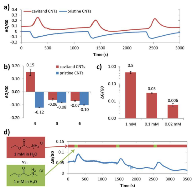
Figure 4. Liquid flow sensing experiments with Tiii@SWCNT -based devices at pH 5. a) Tiii@SWCNT and pristine SWCNTs show opposite responses upon exposure to a 1 mM solution of 4 b) Comparison of the current change upon exposure of Tiii@SWCNT and pristine SWCNTs devices to 4 (sarcosine ethylester hydrochloride), 5 (glycine ethylester hydrochloride) and 6 (tetraethylammonium chloride), error bars are based on three consecutive measurements c) Response of Tiii@SWCNT devices to different concentrations of 4 , error bars are based on three consecutive measurements d) Response of Tiii@SWCNT devices to alternating exposure to 4 and 5
