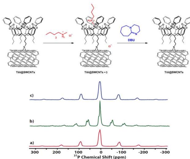
Figure 3. Host-guest binding studies using ^{31}\text{P} MAS NMR showing reversibility of the host molecule. a) Tiii@SWCNTs , (red trace); b) after treatment with 3 (green trace) c) after base treatment (blue trace)
