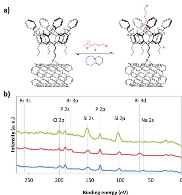
Figure 2. XPS binding study with Tiii@SWCNTs . a) Reversible binding of guest 2 ; b) XPS analysis of Tiii@SWCNTs before exposure to 2 (blue), after exposure to 2 (red) and after subsequent washing with DBU (green). Si signals are due to the utilized Si substrate.
