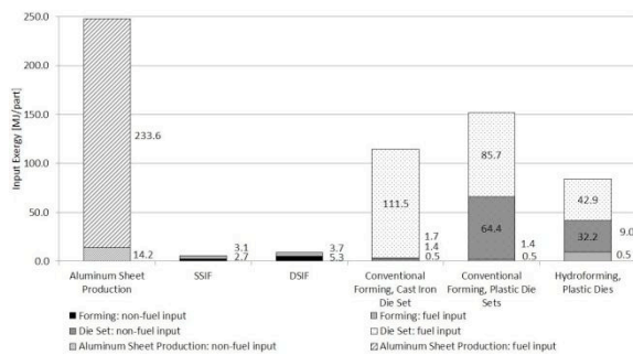
Fig. 9 Comparison of exergy inputs for different forming technologies; batch size: 200 parts; control volume: supply chain
