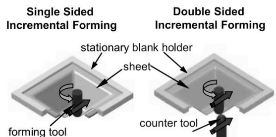
Fig. 1 Single and double sided incremental forming [3]
