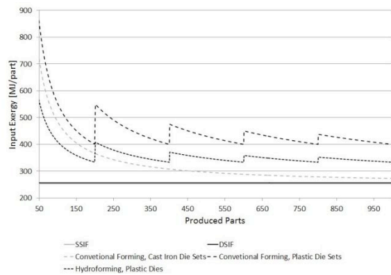
Fig. 8 Comparison of forming related exergy inputs (without aluminum production); control volume: supply chain
