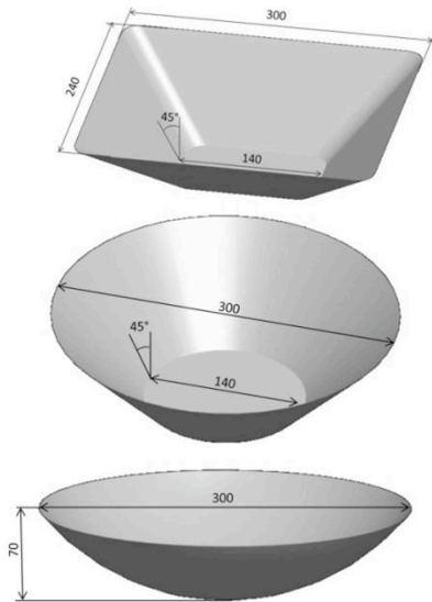
Fig. 2 Sample parts: box, cone and dome
