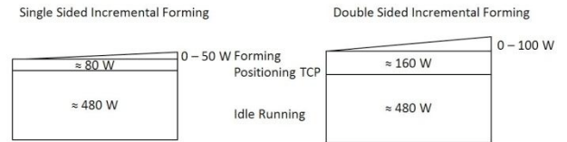
Fig. 3 Results power measurements of SSIF and DSIF
