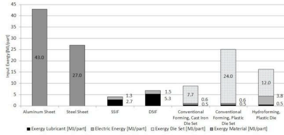
Fig. 6 Comparison of exergy inputs for different forming technologies; batch size: 200 parts; control volume: forming machine
