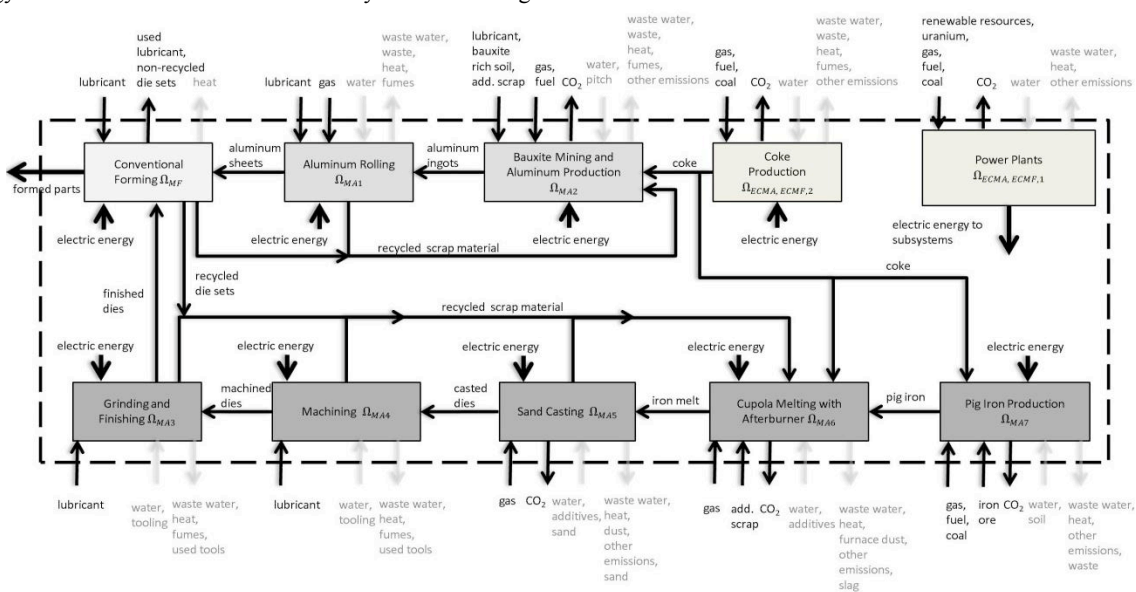
Fig. 7 Control volume of the supply chain for formed aluminum parts with a conventional press and cast iron die sets
