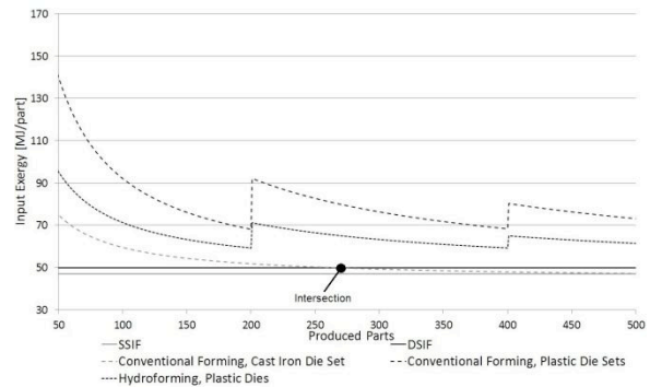
Fig. 5 Exergy inputs over the number of produced aluminum parts; control volume: forming machine
