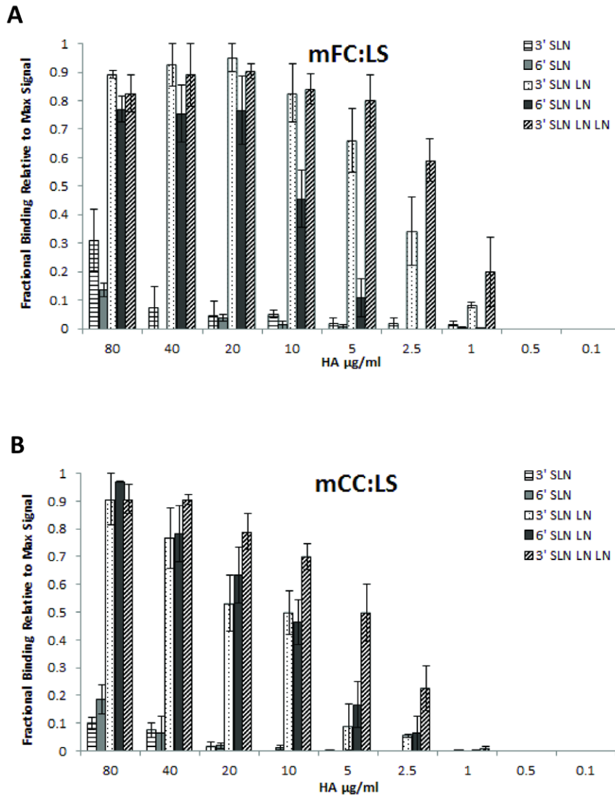
Figure 2. Glycan receptor-binding specificity of Gln226→Leu/Gly228→Ser mutant of FC and CC. A and B, respectively show dose-dependent direct glycan array binding of mFC:LS and mCC:LS mutant HAs. The double mutation leads to a substantial increase in human-receptor binding signals to a level that allowed calculation of apparent binding affinity parameter K_d' . The double mutation also lowers the avian-receptor binding affinity of mutant HAs relative to the corresponding wild-type HAs. doi:10.1371/journal.pone.0049597.g002
