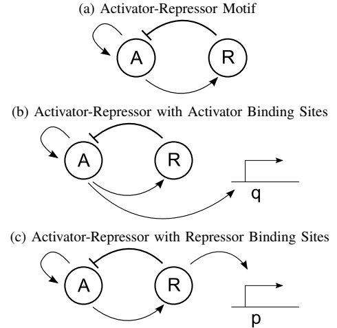
Fig. 1. Diagram (a) illustrates the activator-repressor motif. Diagram (b) and (c) illustrate the systems after the addition of DNA binding sites with affinity to the activator and the repressor respectively.
