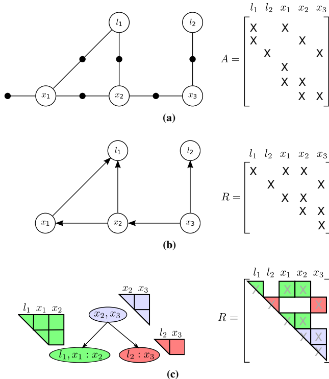
Fig. 3: (a) The factor graph and the associated Jacobian matrix A for a small SLAM example, where a robot located at successive poses x_1 , x_2 , and x_3 makes observations on landmarks l_1 and l_2 . In addition there is an absolute measurement on the pose x_1 . (b) The chordal Bayes net and the associated square root information matrix R resulting from eliminating the factor graph using the elimination ordering l_1, l_2, x_1, x_2, x_3 . The last variable to be eliminated, here x_3 , is called the root. (c) The Bayes tree and the associated square root information matrix R describing the clique structure in the chordal Bayes net. A Bayes tree is similar to a junction tree, but is better at capturing the formal equivalence between sparse linear algebra and inference in graphical models. The association of cliques and their conditional densities with rows in the R factor is indicated by color.
