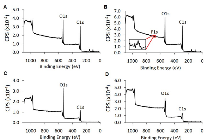
Figure 2. XPS spectra of electrospun fibers. (A) PCL, (B) PCL/dex, (C) PLLA, and (D) PLLA/dex. CPS stands for counts per second.
