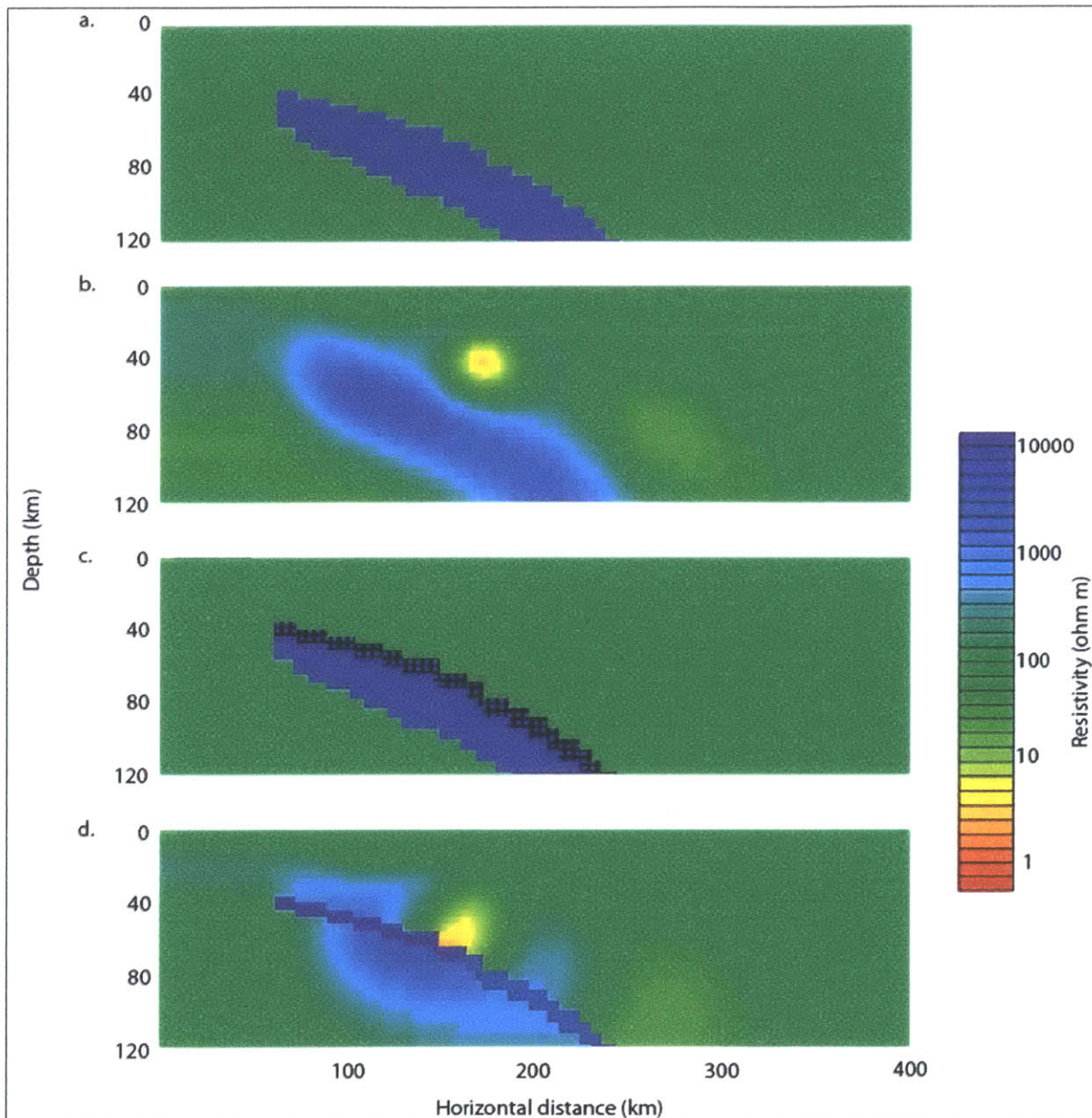
Figure 15: Figure 14 shows the impact of an assumption in which the top of the resistive dipping feature is placed approximately 10 km too low in the starting model (again based on synthetic data generated from the forward model in figure 12a). The inversion in figure 14b moves the resistive feature shallower, though it also exhibits “retreat” from the conductive feature as described in Chapter 4. The starting model in figure 14c includes an imposed tear zone, and the associated inverted model is shown in figure 14d. In this case, the resistive feature passes the tear zone boundary and extends upwards. These kinds of analyses show that examining starting models with combinations of imposed features and tear zones, we can determine with some confidence both the accuracy of our assumptions and the manner in which they might not be correct.
