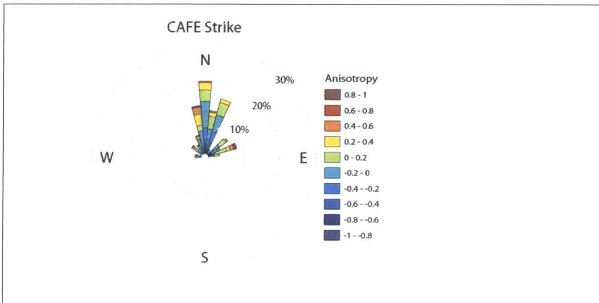
Fig 5: Rose diagram showing overall strike directions with the color code reflecting the degree of anisotropy as determined using the STRIKE algorithm for the CAFE data set (McNeice and Jones, 2001).
