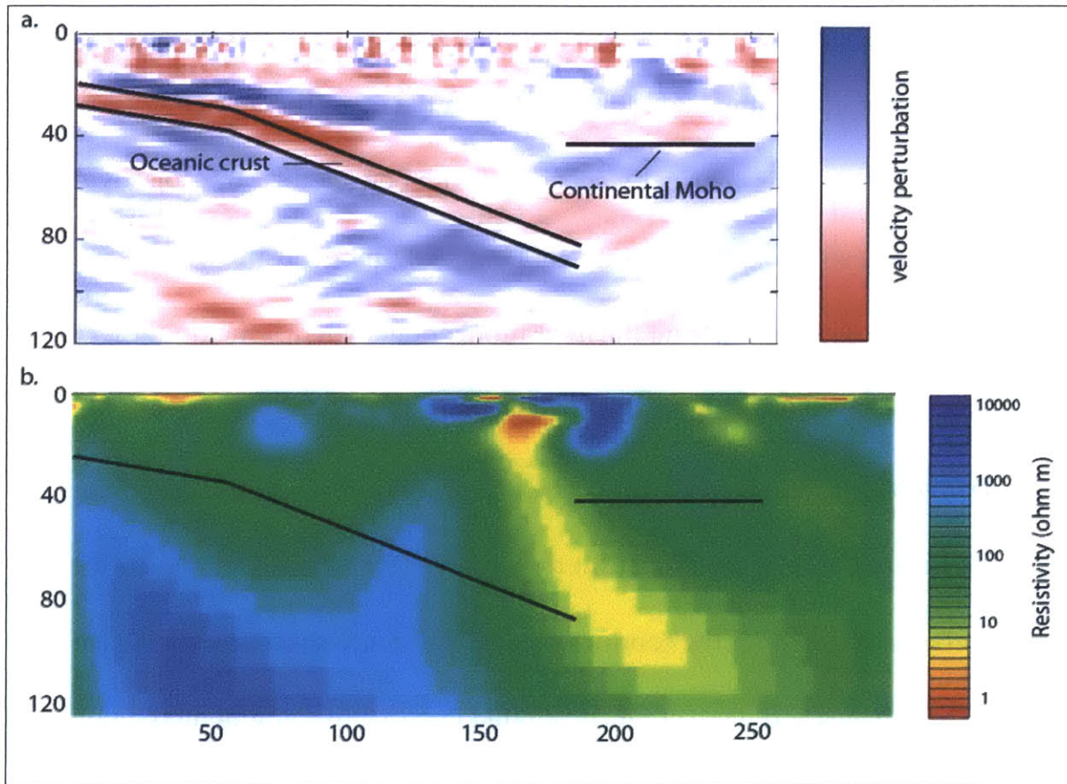
Figure 7: Primary images from the teleseismic migration (fig. 7a) and magnetotelluric (fig. 7b) studies from the previous chapters.
