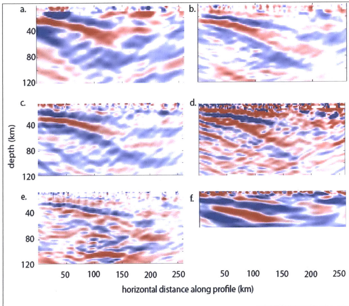
Figure 3: Raw sections for the CAFE line migration. Figure 3a is the primary \delta\alpha/\alpha image for the set, and figure 3b is the primary composite \delta\beta/\beta image, composed of the backscattered PS (figure 3c), the backscattered SSv (figure 3d), the backscattered SSh (figure 3e), and the forward scattered PS (figure 3f) modes.
