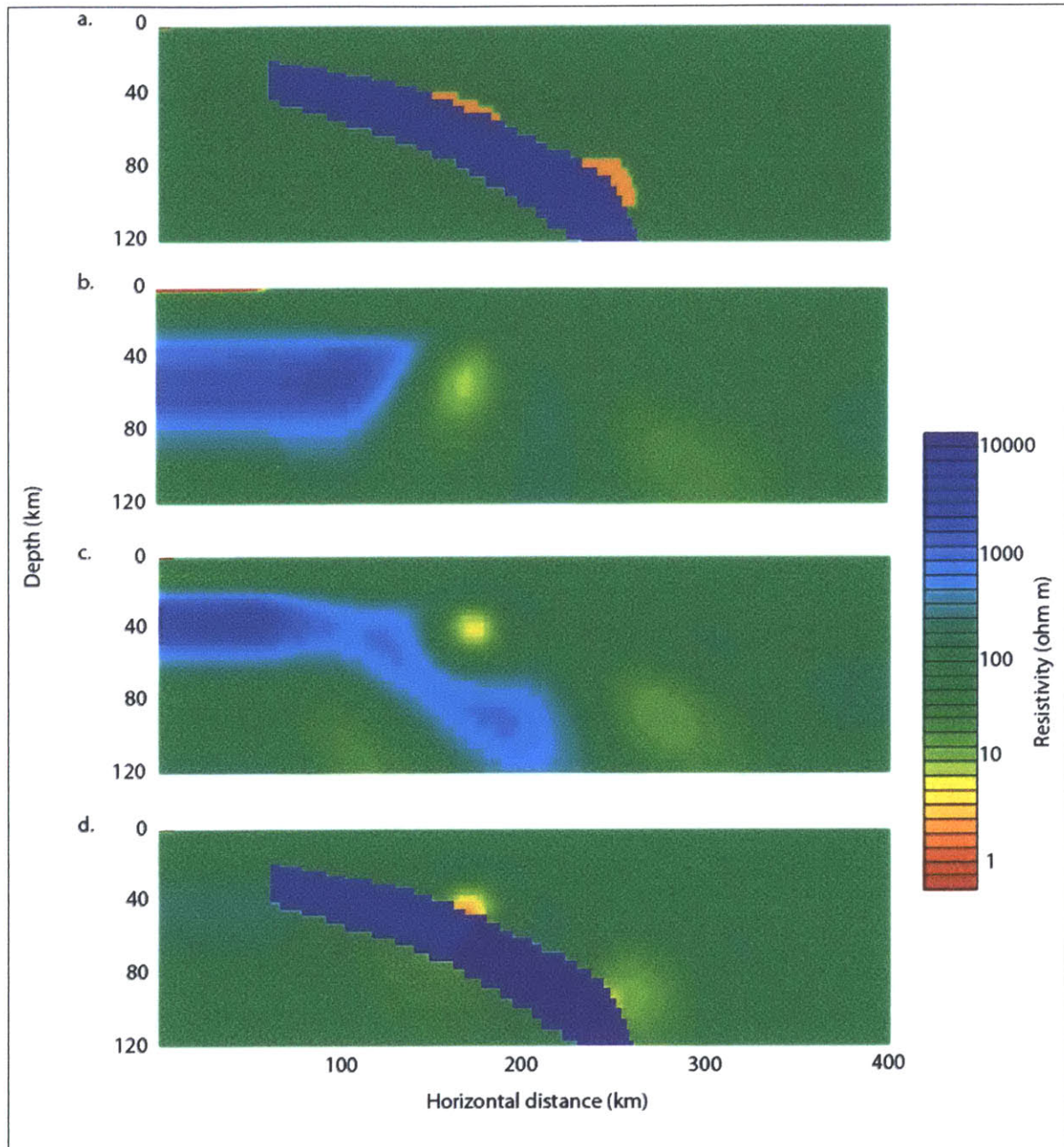
Figure 2: Inversion model for a subducting slab with thin conductors at depths corresponding to fluid release from dehydration reactions for Cascadia. Fig. 2a shows the forward model. Fig. 2b shows the inversion model from a halfspace. Fig. 2c shows the inversion model with the resistive slab imposed into the starting model. Fig. 2d shows the inversion model with the imposed resistive slab and a tear zone incorporated into the slab.
