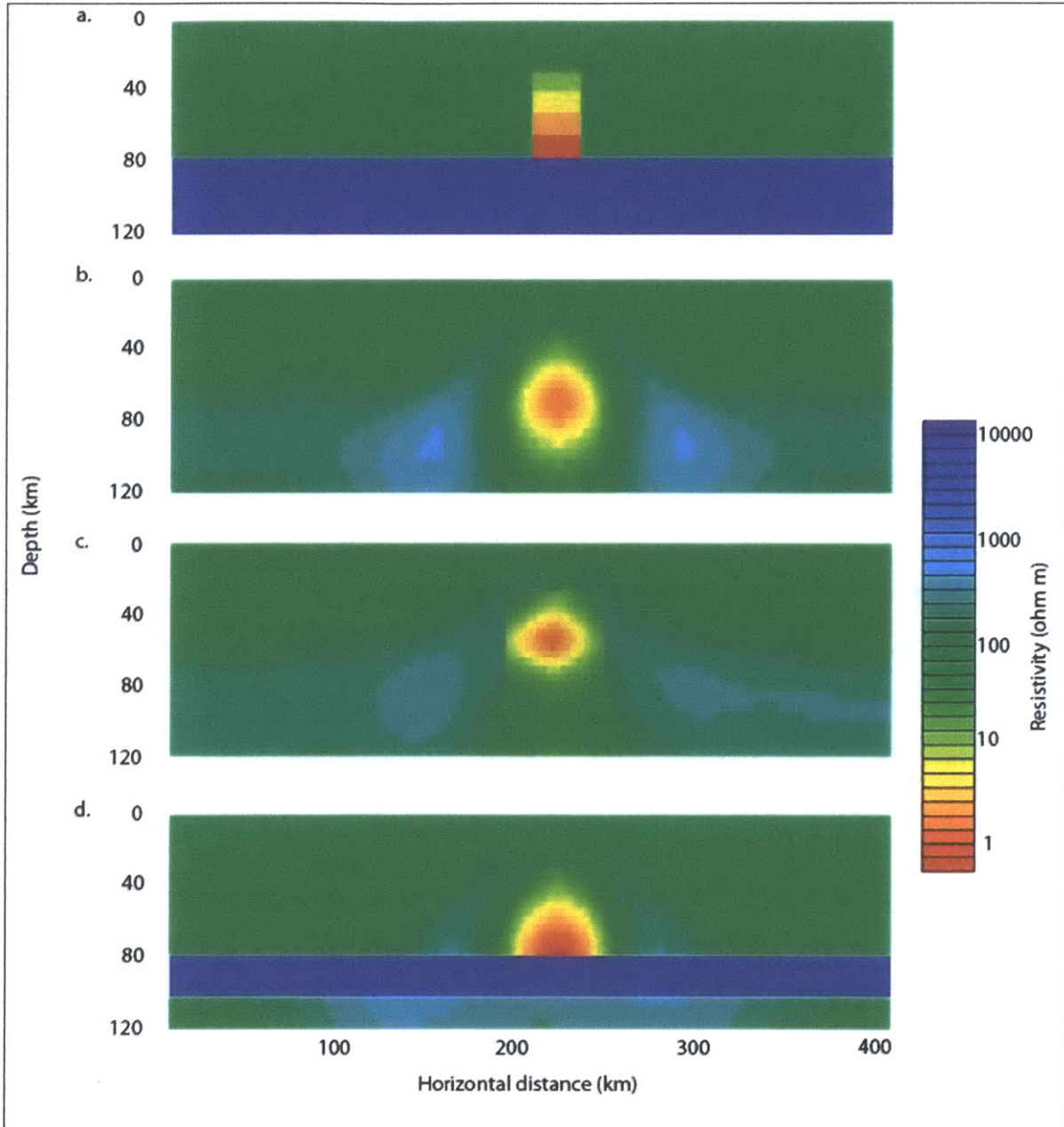
Figure 5: Inversion models demonstrating the loss of detail in a conductor with a gradient. Fig. 5a shows the forward model. Fig. 5b shows the halfspace inversion. Fig. 5c shows an inversion with a tear zone imposed over the region of the conductor, and Fig. 5d an inversion model with both an imposed resistive layer and tear zone over the resistive layer.
