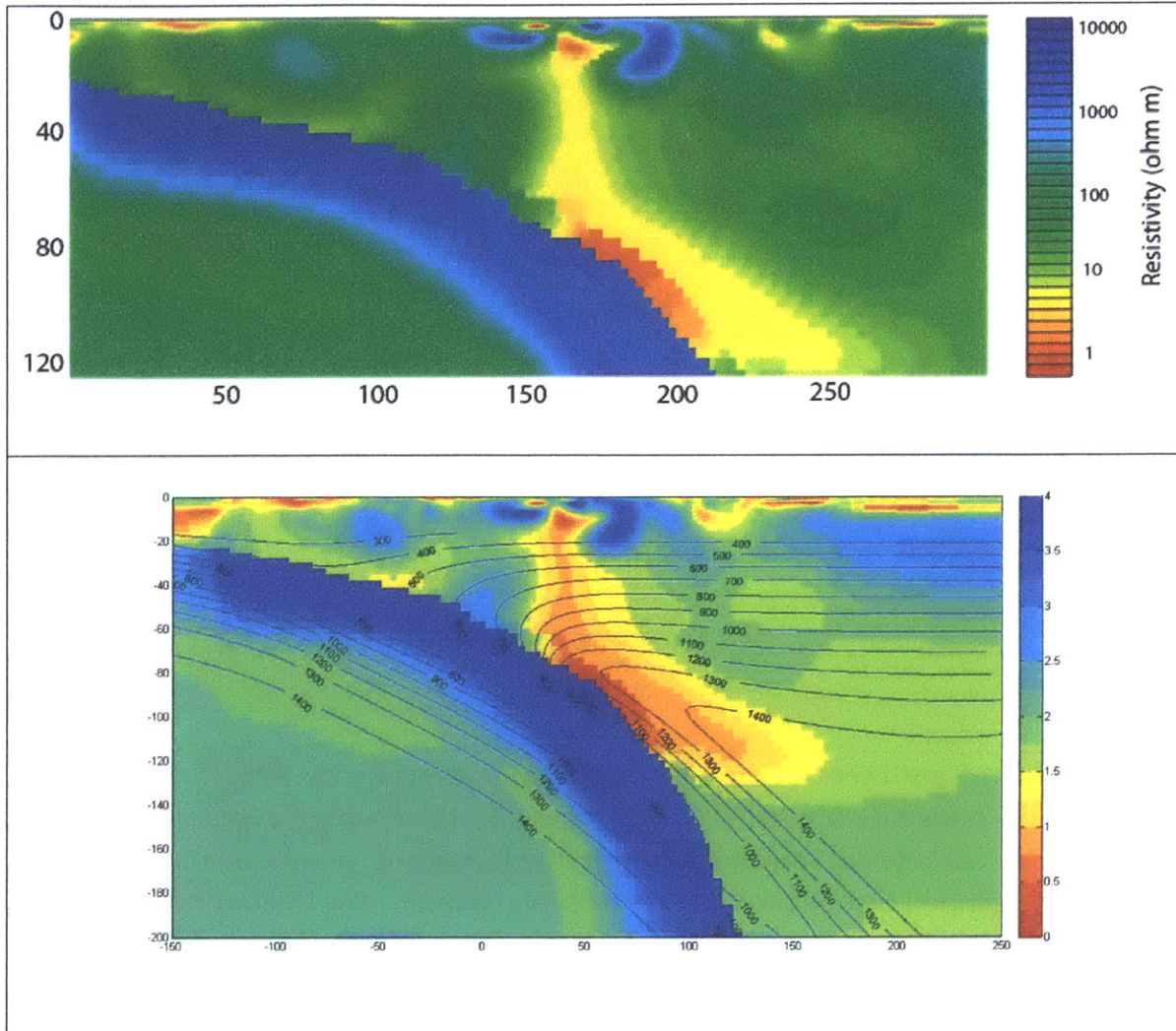
Figure 8: The top panel shows the augmented MT inversion model incorporating a priori information using the methods developed in section 4. In the lower panel, a thermal profile for the Cascades (van Keken, 2011) is superimposed on the model. Note that the thermal model assumes a shallower dip angle for the slab in the eastern part of the model.
