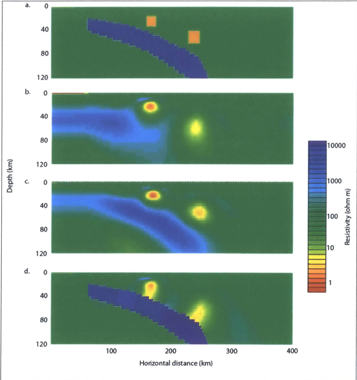
Figure 3: Inversion model for a subducting slab with conductors separated from the top of the slab. Fig. 3a shows the forward model. Fig. 3b shows the inversion model from a halfspace. Fig. 3c shows the inversion model with the resistive slab imposed into the starting model. Fig. 3d shows the inversion model with the imposed resistive slab and a tear zone incorporated into the slab.
