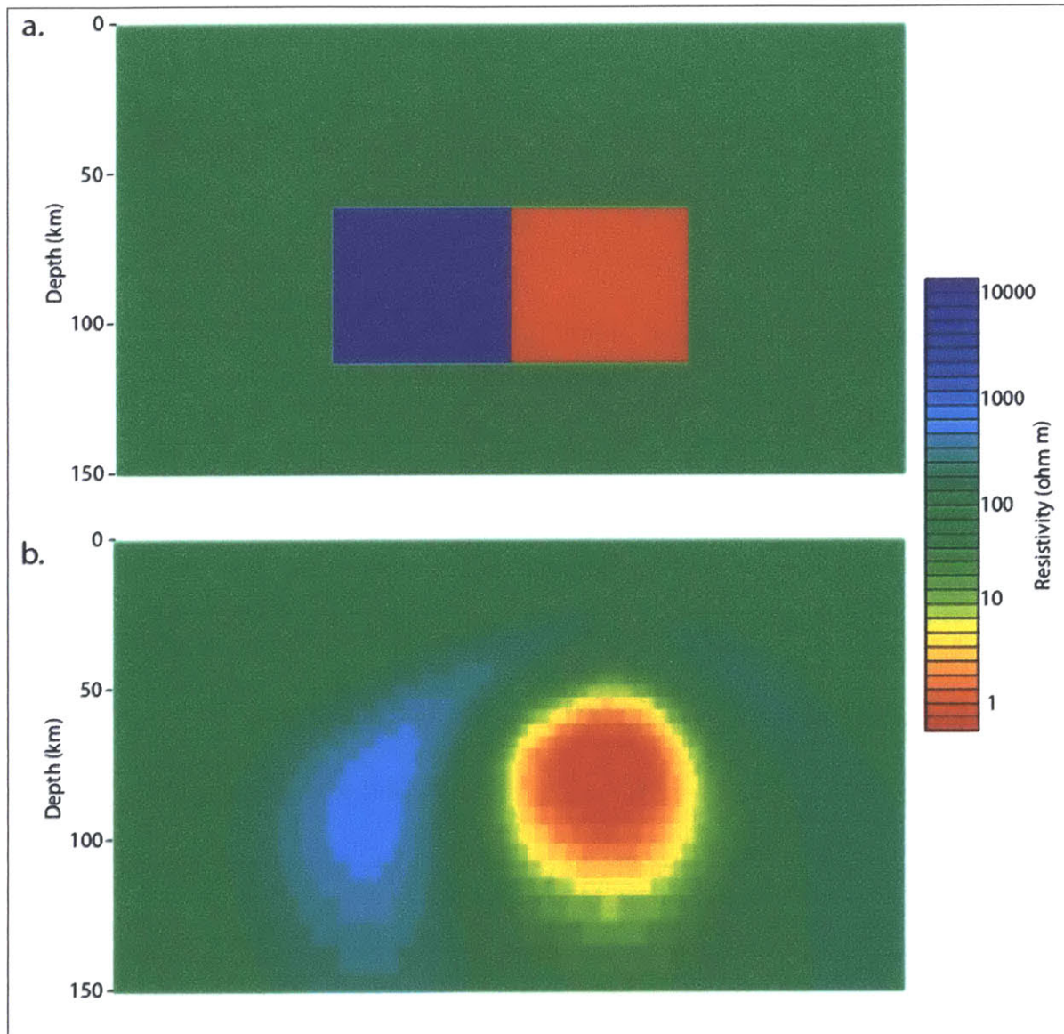
Figure 1: Inversion model demonstrating the effect of a smoothing stabilizing functional for a simple two block model. Figure 1a shows the forward model, which was also used as the starting model, and Figure 1b shows the inversion.
