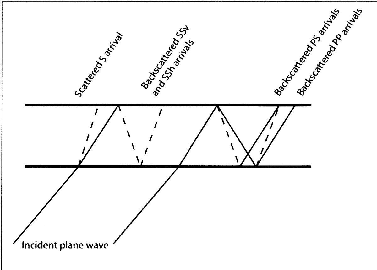
Figure 1: A simple illustration of the modes used for the migrated sections in this paper. The incident plane P-wave encounters a scattering contact in the subsurface, such that the energy of the transmitted wave is divided into P wave components (solid lines) and S wave components (dashed lines). The \delta\alpha/\alpha (P-wave) sections show the backscattered PP mode in isolation, whereas the \delta\beta/\beta (S-wave) sections show composite images that incorporate the forward PS, and backscattered PS, SSv, and SSh modes. The SSv and SSh modes differ only in polarization, with the SSv being the component of the wave polarized in the vertical, and SSh being the component polarized in the horizontal.
