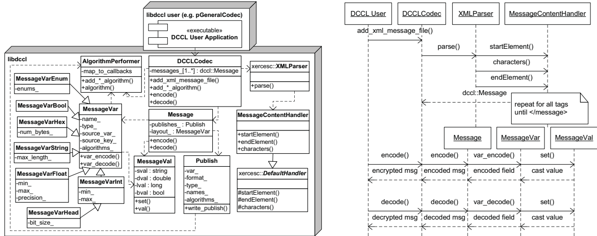
(a) Structure diagram. Dependencies between classes are indicated by a dashed arrow. Class generalizations are indicated with a solid arrow (e.g. MessageVarInt is a MessageVar).
