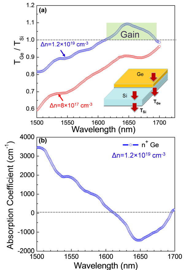
FIG. 3. (a) Transmittance spectra through the n^+ Ge-on-Si sample in reference to the Si substrate under the injection levels of 1.2 \times 10^{19} \text{ cm}^{-3} and 8 \times 10^{17} \text{ cm}^{-3} . T_{\text{Ge}} and T_{\text{Si}} refer to the transmittance through the n^+ Ge-on-Si sample and the Si substrate alone, respectively. (b) Derived absorption spectrum of the n^+ Ge sample under 1.2 \times 10^{19} \text{ cm}^{-3} carrier injection.
