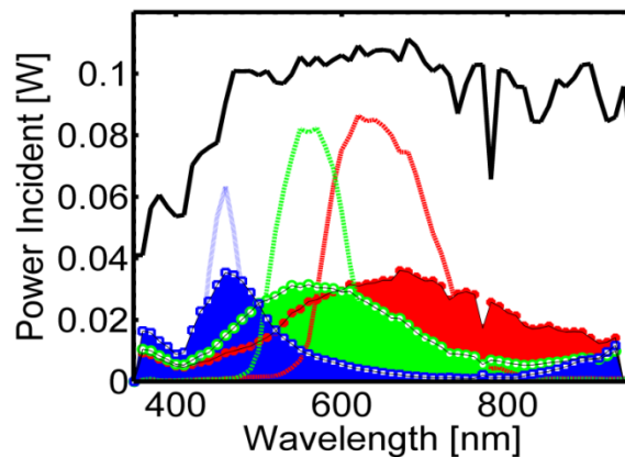
Fig. 5. Simulated (dashed lines) and experimental (full area curves) power distribution for 3 different positions of the integrating sphere.
