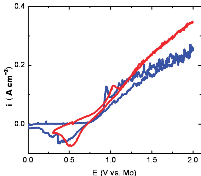
Figure 1. (Color online) CVs of an Ir wire (diameter 0.5 mm) working electrode in molten S1 [MgO(16 wt %)-CaO(18 wt %)-Al 2 O 3 (20 wt %)-SiO 2 (46 wt %)] without (blue line) and with 5 wt % FeO (red line) at 1575°C with a potential scan rate of 100 mV/s, reference electrode and counter electrode: Mo rods (3.17 mm in diameter).
