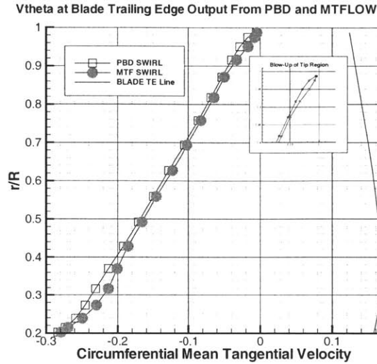
Figure 6-3: The circumferential mean tangential velocity at the blade trailing edge position output from PBD and MTFLOW. They are not equal due because the blade circulation extends beyond the blade tip, overpowering the fluid. Hence the overall strength of the swirl (circulation) was decreased to account for this effect
