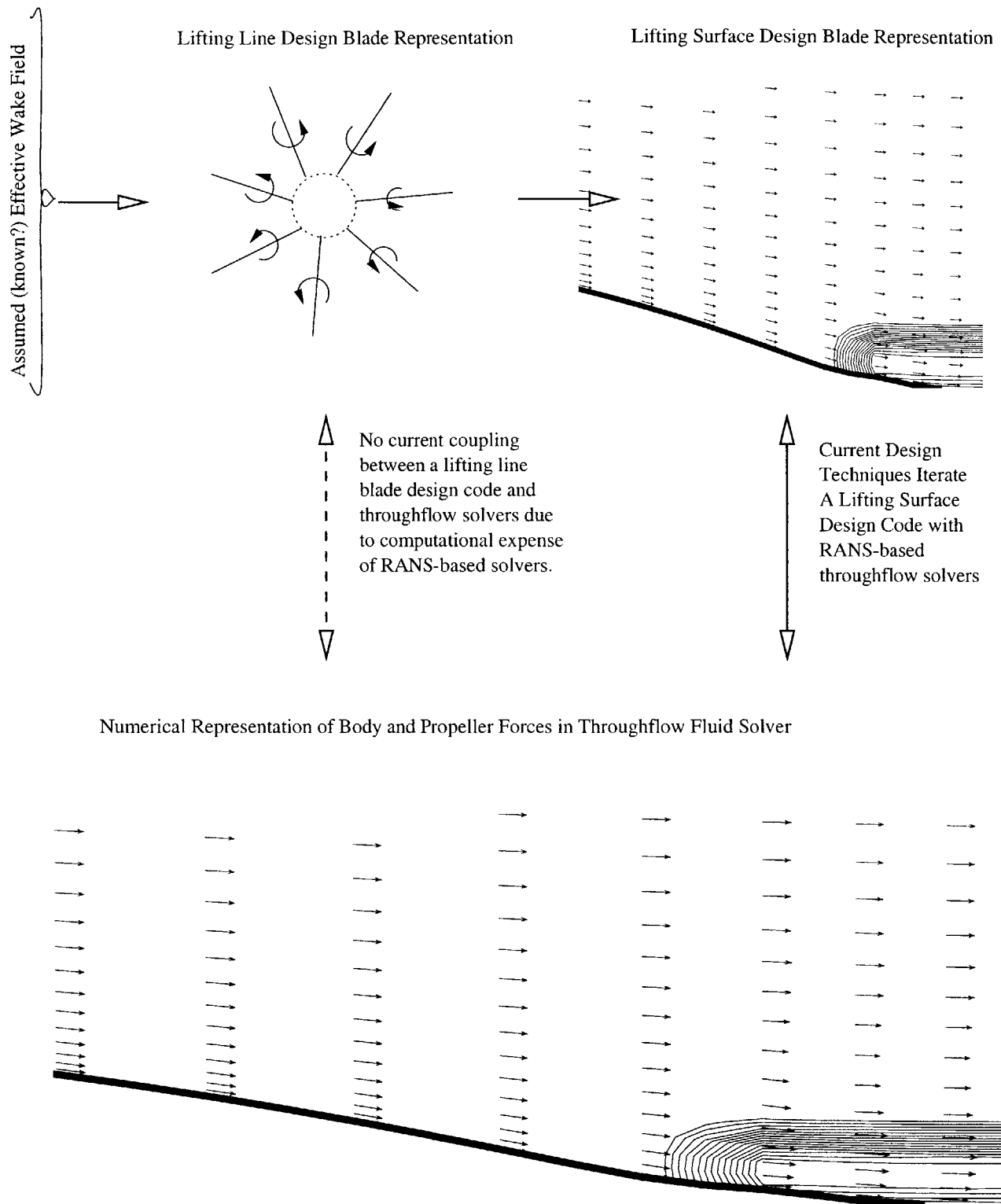
Figure 1-2: The preliminary propeller design process relies upon an assumed effective wake ( i.e. , velocity field) as input to a lifting line analysis to optimize the propeller and lifting surface analysis to design the three dimensional blade shapes. There is a limited amount of coupling with throughflow solvers to iterate upon the effective wake.
