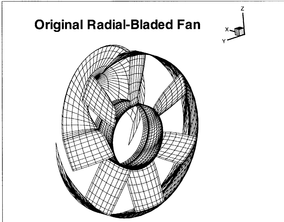
Figure 7-3: The original radial fan with cut-away duct. The trailing wake vortex system is shown emanating only from one blade to maintain clarity.
