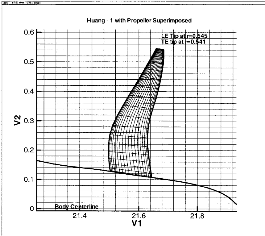
Figure 6-9: Huang Body 1 Stern Profile with Propeller 4577
