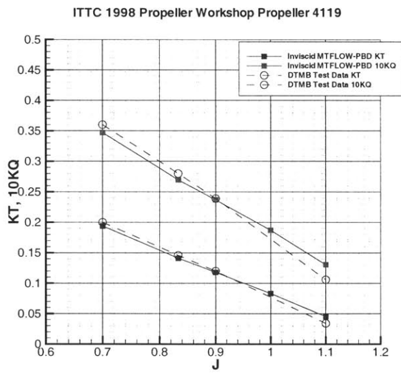
Figure 6-11: comparison of MTFLOW-PBD with P4119 ITTC Test.
