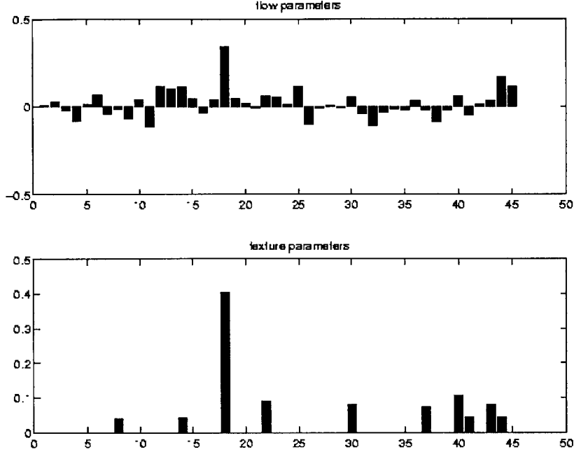
Figure 6-4: Top: Analyzed \alpha_i flow parameters computed for one image. Bottom: The corresponding analyzed \beta_i texture parameters computed for the same image. The \beta_i texture parameters are typically zero for all but a few image prototypes.
