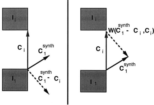
Figure 6-2: The flow reorientation process: First, C_i is subtracted from the synthesized flow C_1^{synth} . Second, this flow vector is itself forward warped along C_i .
