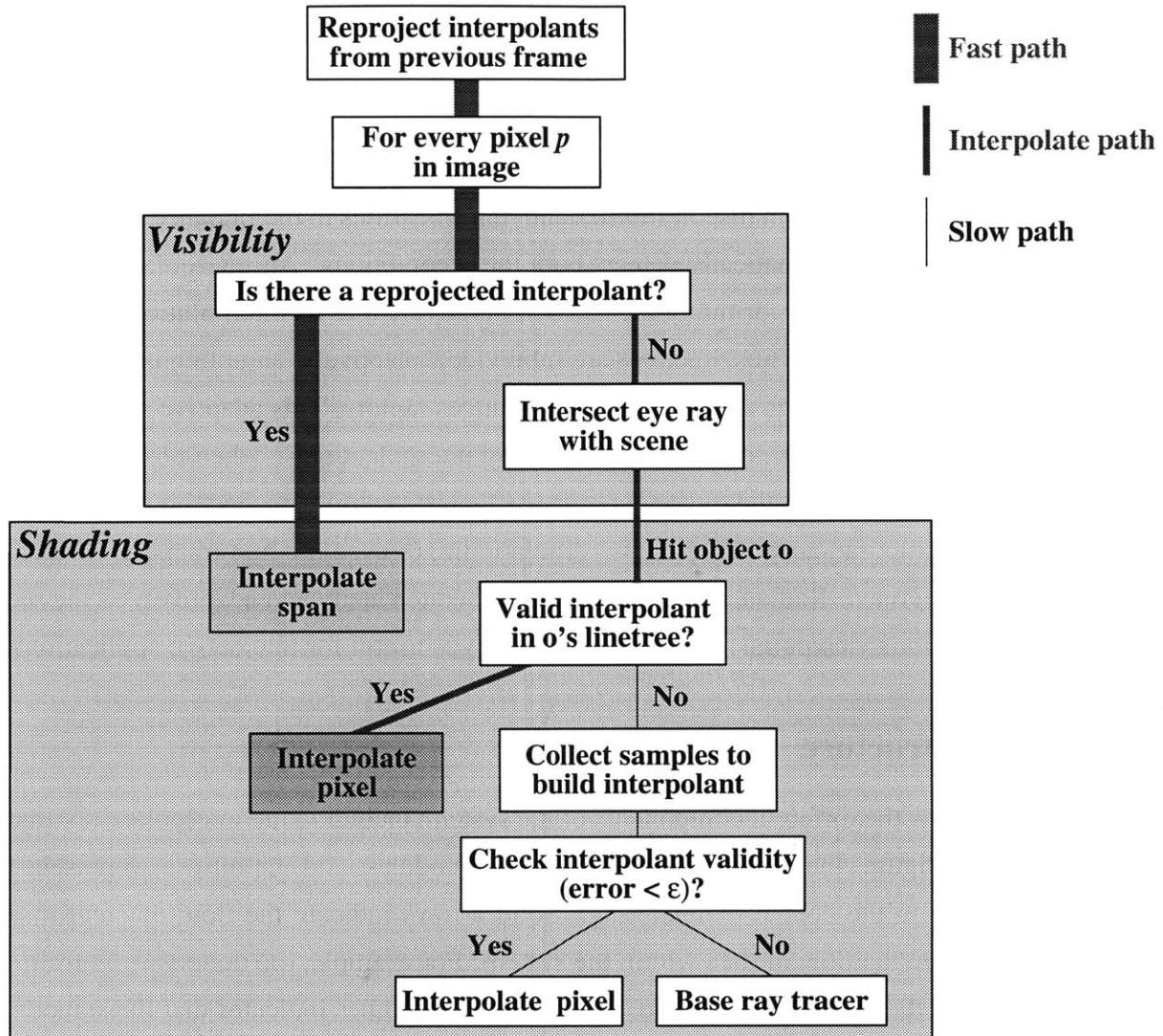
Figure 1-5: Algorithm overview.
