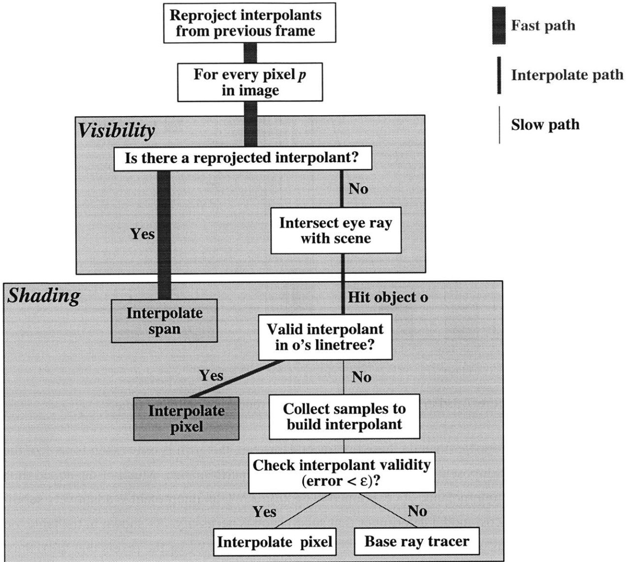
Figure 7-2: Algorithm overview.
