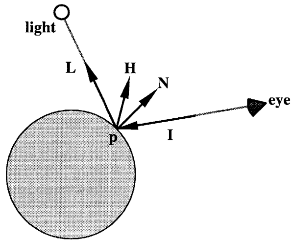
Figure 4-18: Ray geometry.
