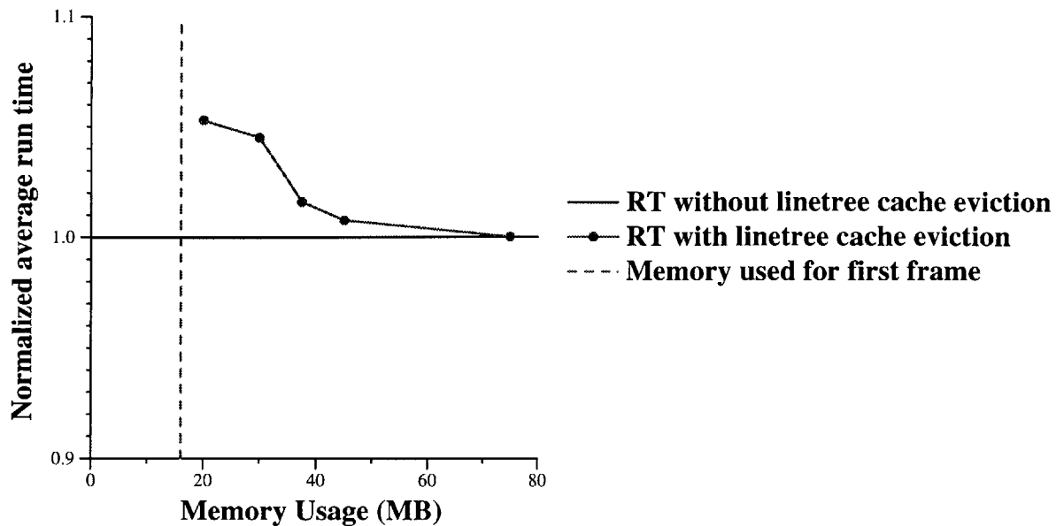
Figure 7-5: Impact of linetree cache management on performance.
