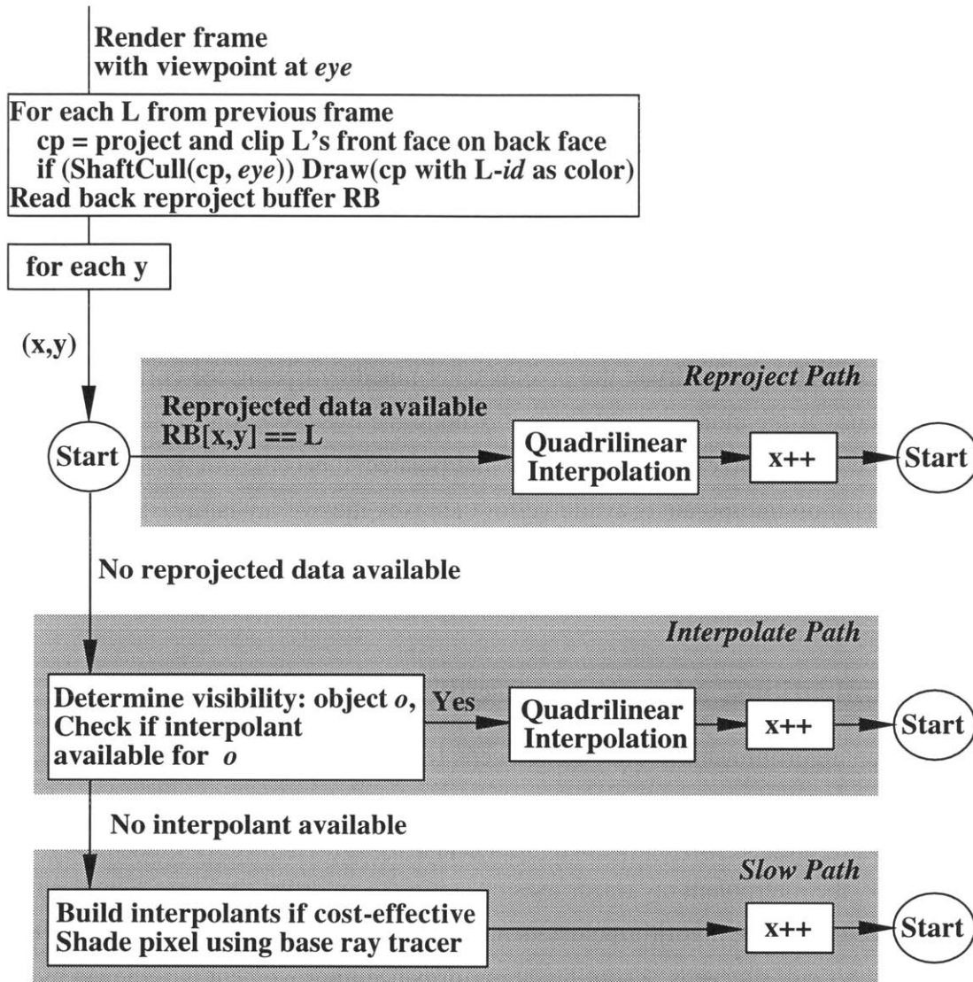
Figure 5-6: Reprojection algorithm.
