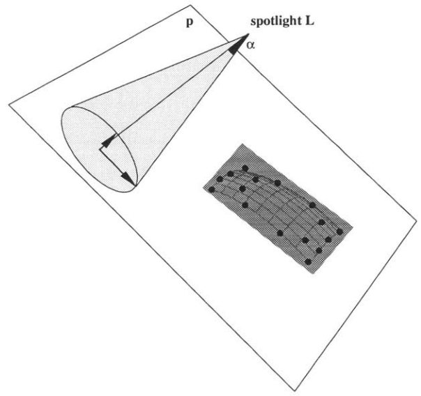
Figure 4-15: Spotlight: Test 4.
