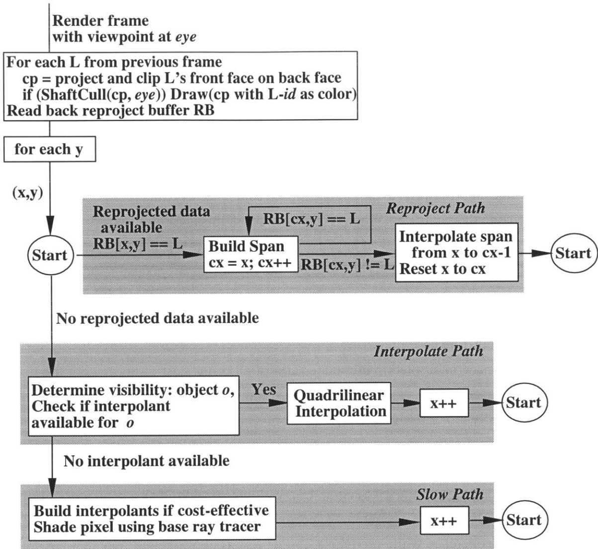
Figure 5-7: Reprojection algorithm with screen-space interpolation.
