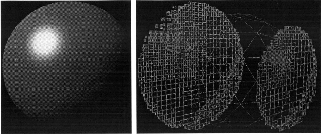
Figure 3-9: Linetree visualization. On the left is an image of a sphere rendered using the interpolant ray tracer. On the right is a visualization of the corresponding linetree cells.
