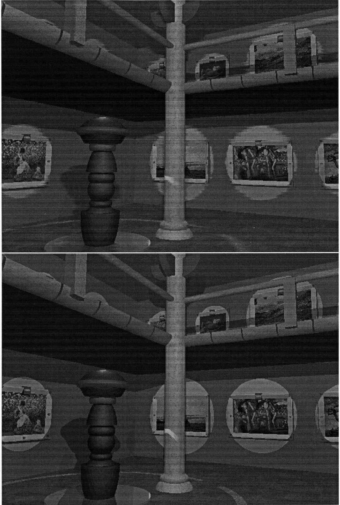
Figure 5-11: Extrapolation for the museum scene. Top: Algorithm 3, matching visibility. Bottom: Algorithm 4, matching ray trees.
