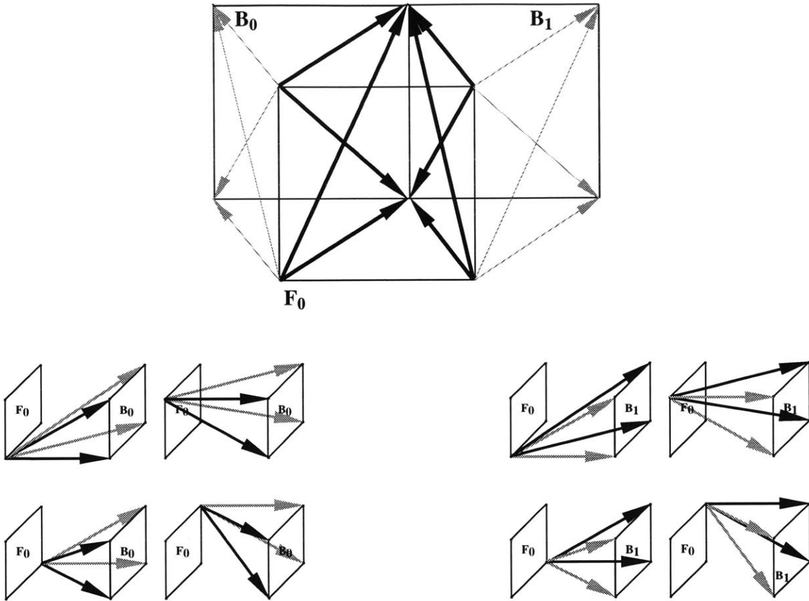
Figure 3-12: Common rays.
