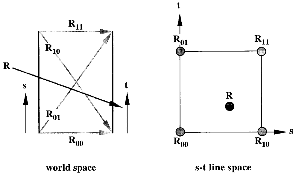
Figure 3-5: A segment pair and its associated s - t line space.
