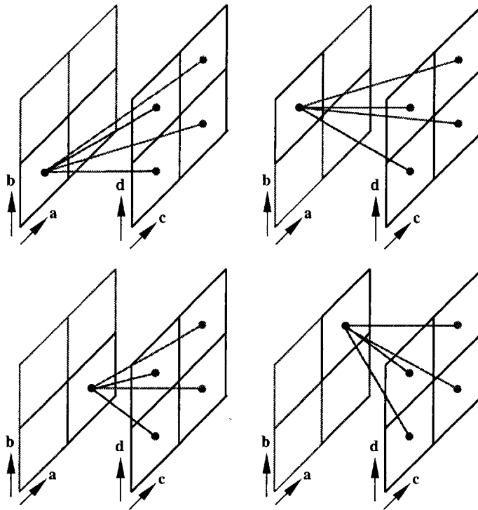
Figure 3-8: Linetree cell subdivision.
