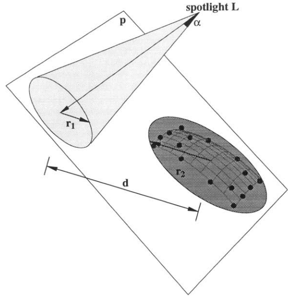
Figure 4-13: Spotlight: Test 2.
