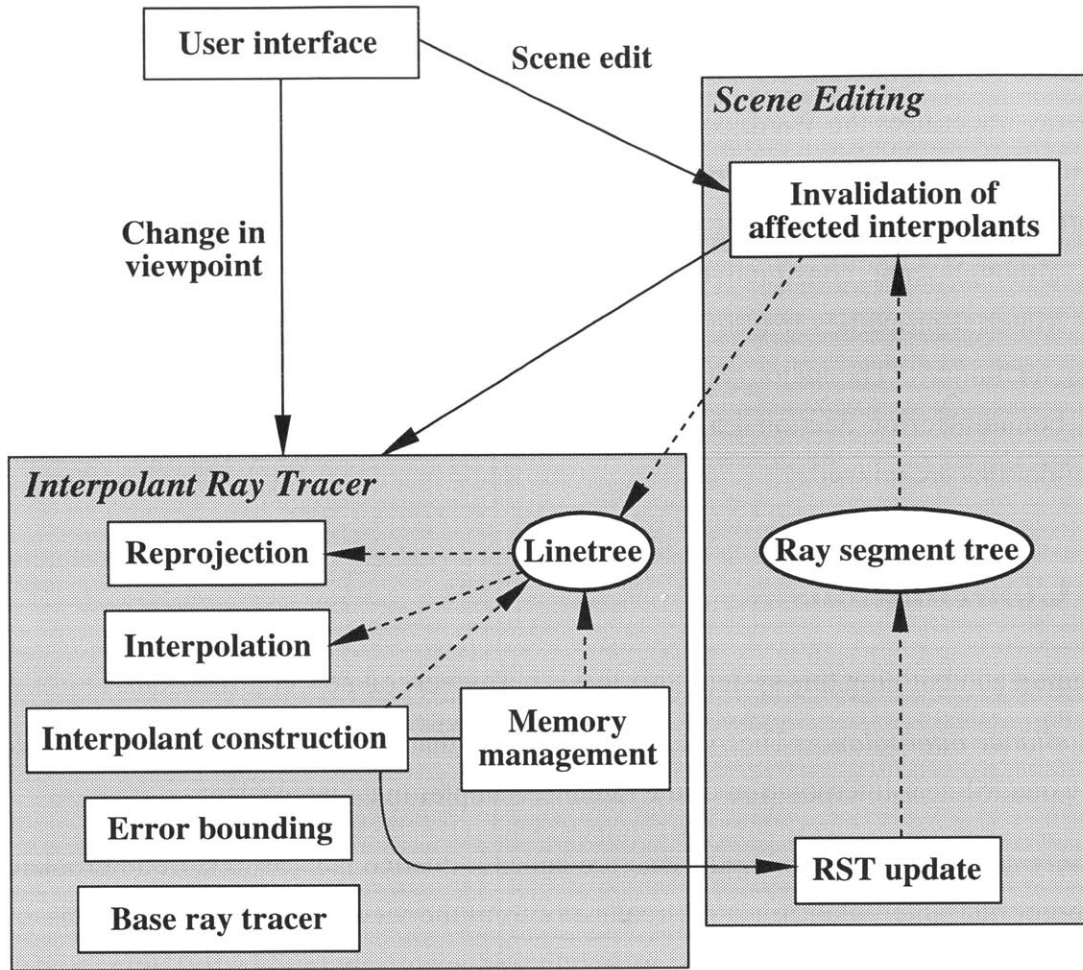
Figure 1-6: System overview.
