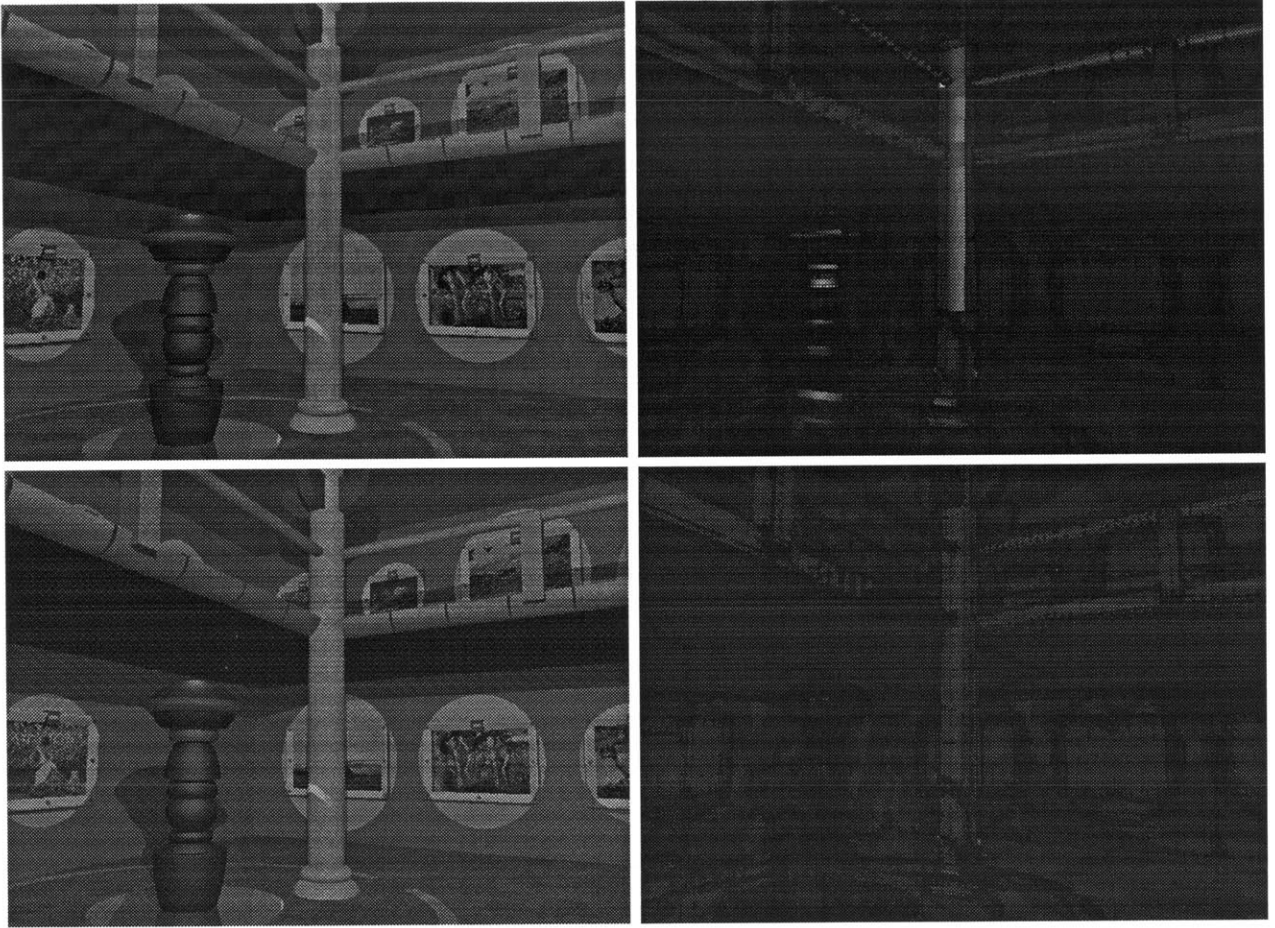
Figure 4-27: Error refinement for the museum scene. Top row: without non-linearity detection. Bottom row: with non-linearity detection and \epsilon = 0.5 . Right column: scaled difference images.
