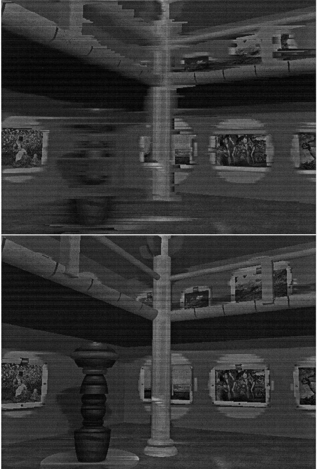
Figure 5-10: Extrapolation for the museum scene. Top: Algorithm 1 (simple extrapolation), Bottom: Algorithm 2 (extrapolation with correct visibility).
