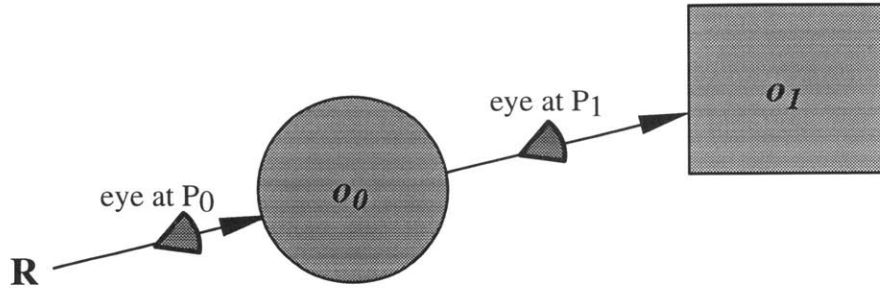
Figure 3-4: Radiance along ray \mathbf{R} depends on the eye position.
