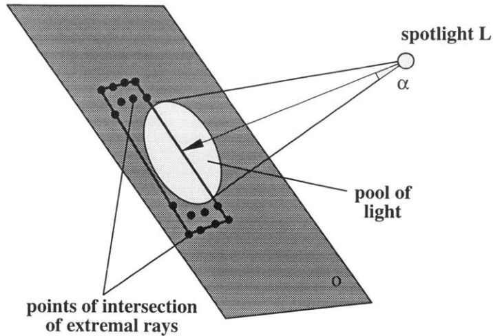
Figure 4-11: Problem with spotlights.
