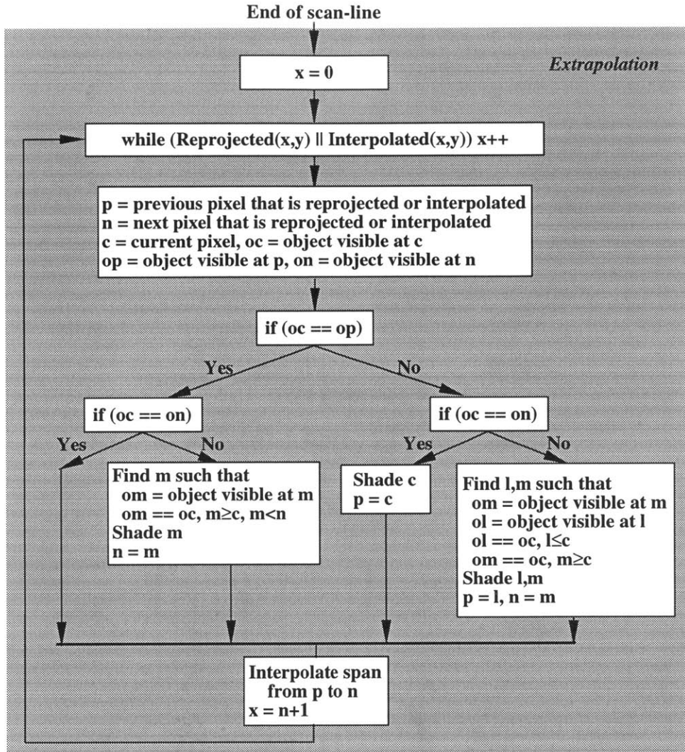
Figure 5-9: Algorithm 2: extrapolation with correct visibility determination.
