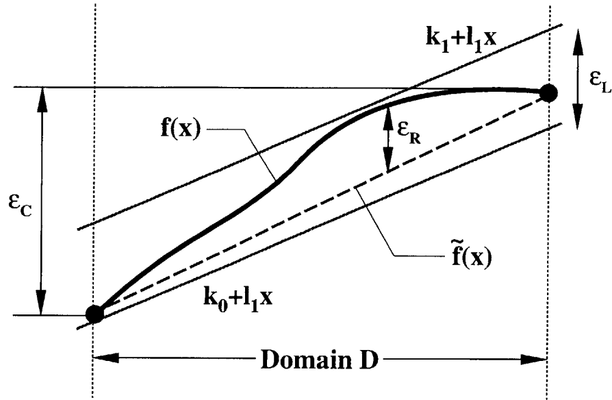
Figure 4-19: Interpolation error. The thick black curve is the base radiance function f(x) . The dark shaded circles at the end-points of the domain D are the samples that are interpolated, and the dotted line at the bottom of the curve is the interpolated radiance function \tilde{f}(x) . \epsilon_R is the interpolation error, \epsilon_C is the error computed by standard (constant) interval arithmetic, and \epsilon_L is the error computed by linear interval arithmetic.
