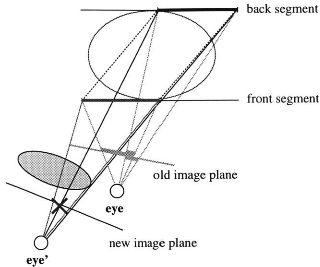
Figure 5-4: Reprojection correctness. The shaded ellipse occludes visibility to the linetree cell from the new viewpoint eye' but not from eye . Therefore, it would be incorrect to reproject the linetree cell to the new viewpoint.
