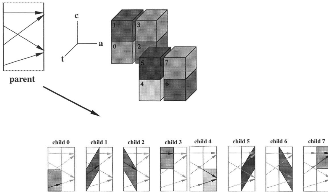
Figure 6-10: Subdivision of ray segment trees.
