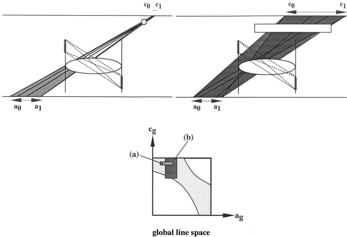
Figure 6-7: Global line space for: (a) light rays, (b) reflected rays.
