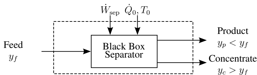
Figure 2. A control volume for an arbitrary black box chemical separator powered by work only.
