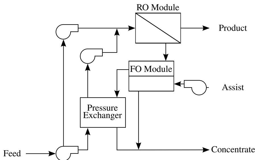
Figure 10. Schematic diagram of a typical single stage reverse osmosis system with a forward osmosis and pressure exchanger energy recovery devices.
