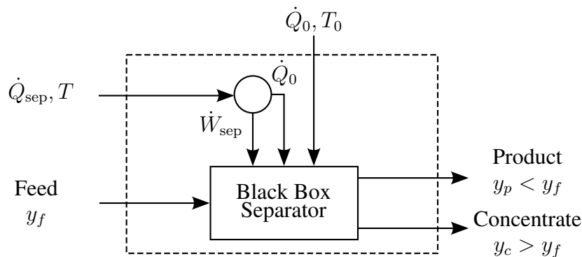
Figure 4. A control volume for an arbitrary black box chemical separator when heat is the only form of energy input.
