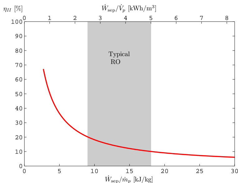
Figure 15. The Second Law efficiency of a work-driven desalination system operating in a cogeneration scheme can never reach 100% unless the power plant operates reversibly. Typical values for current reverse osmosis systems are highlighted. Feed water is at T_0 = 25\text{ °C} and y_f = 35\text{ g/kg} .
