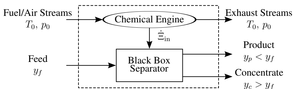
Figure 7. A control volume for an arbitrary black box chemical separator when fuel is the only form of energy input.
