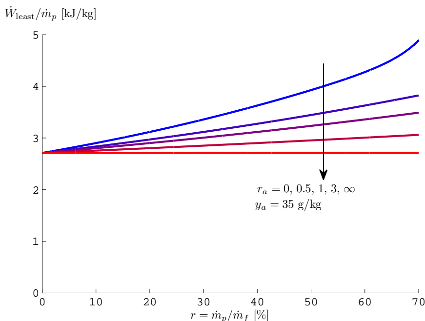
Figure 12. Least work of separation for a black box separator with a salinity gradient engine as a function of feed salinity, recovery ratio, and ratio of the energy recovery stream to the feed. Feed water is at T_0 = 25\text{ }^\circ\text{C} and y_f = 35\text{ g/kg} .
