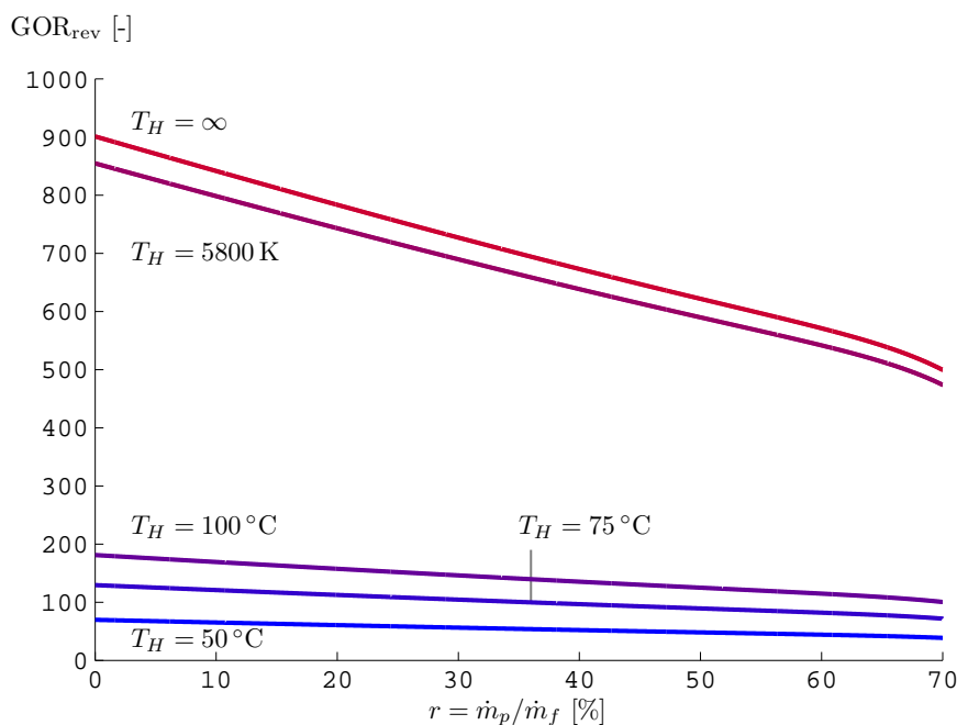
Figure 6. Maximum gained output ratio (GOR) for desalination processes with various temperatures of heat input. Feed water is at T_0 = 25\text{ }^\circ\text{C} and y_f = 35\text{ g/kg} .
