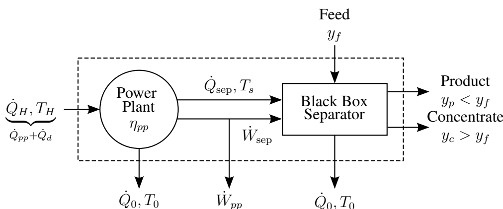
Figure 14. The power plant converts heat input into work output, work for the desalination plant, and heat for the desalination plant. It is assumed that the power plant operates at a Second Law efficiency of \eta_{pp} .
