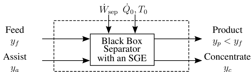
Figure 11. A control volume for an arbitrary black box chemical separator powered by work and a salinity gradient engine.
