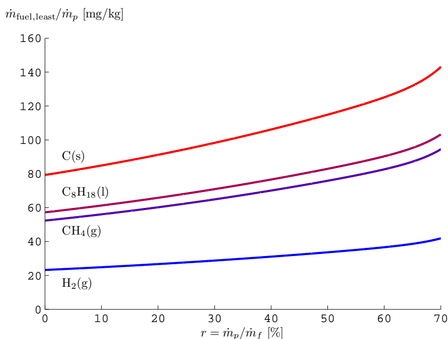
Figure 8. Least amount of fuel needed when using combustion as a function of fuel type and recovery ratio. Feed water is at T_0 = 25\text{ °C} and y_f = 35\text{ g/kg} .
