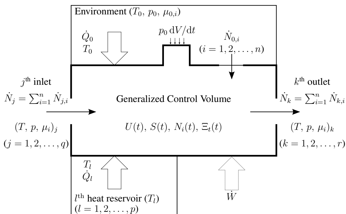
Figure 1. A generalized control volume with q inlets, r outlets, p heat transfer inputs, and work input. The control volume can exchange work ( p_0 dV/dt ), heat ( \dot{Q}_0 ), and mass ( \dot{N}_{0,i} ) with the environment through the system boundary.
