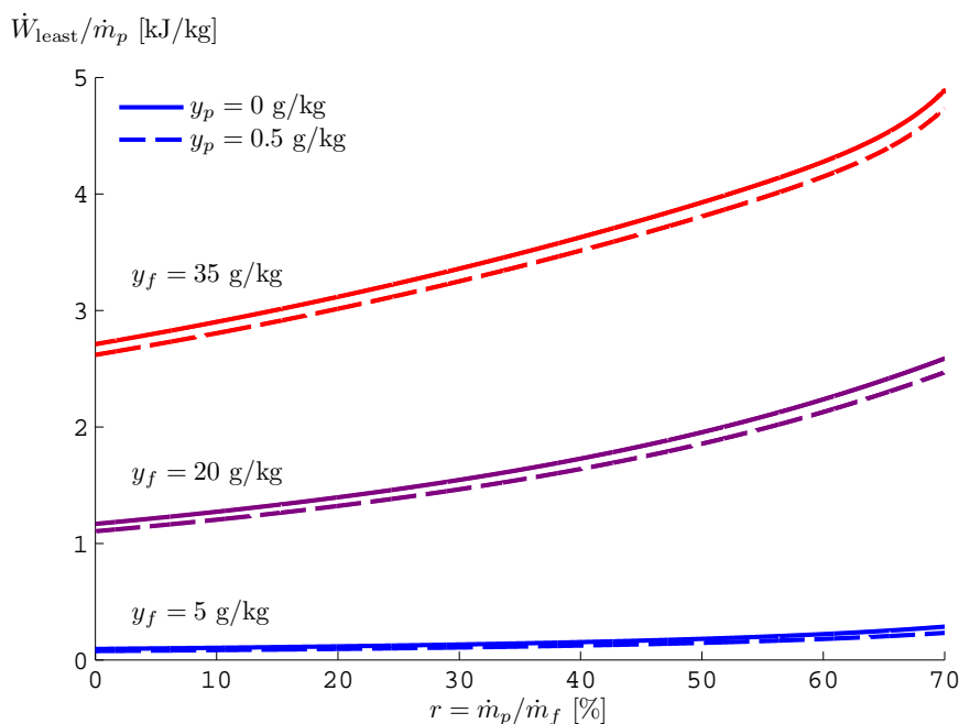
Figure 3. Least work of separation as a function of feed salinity and recovery ratio. Feed water is at T_0 = 25\text{ }^\circ\text{C} .
