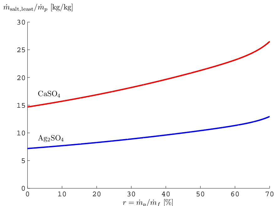
Figure 9. Least amount of salt needed when letting a salt dissociate to equilibrium as a function of recovery ratio for \text{CaSO}_4 and \text{Ag}_2\text{SO}_4 . Feed water is at T_0 = 25^\circ\text{C} and y_f = 35\text{ g/kg} .
