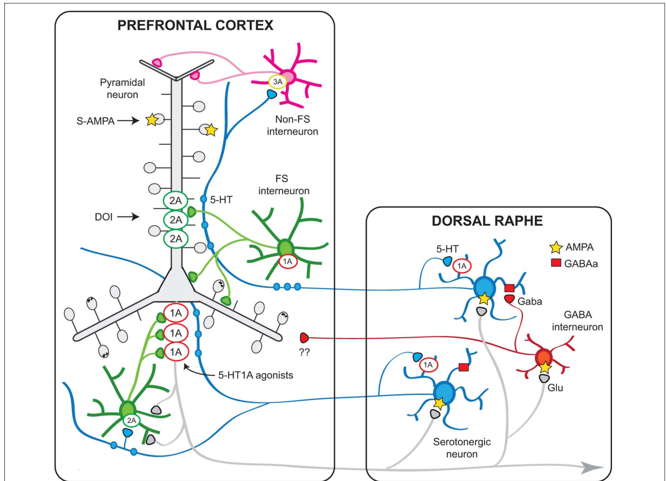
FIGURE 9 | Schematic representation of the relationships between the mPFC and the DR involving 5-HT 1A and 5-HT 2A receptors. Pyramidal neurons in the mPFC project densely to the DR/MnR and modulate the activity of serotonergic neurons via direct and indirect influences (Celada et al., 2001). In turn, endogenous 5-HT modulates pyramidal cell activity through the activation of various receptors expressed in the neocortex, of which 5-HT 1A and 5-HT 2A receptors play a major role. The latter receptors are particularly enriched in apical dendrites of pyramidal neurons where they can facilitate AMPA inputs. A smaller population of 5-HT 2A receptors are expressed by GABA interneurons, including fast-spiking (FS) interneurons. Pyramidal 5-HT 1A receptors may be localized in the axon hillock, together with GABA A receptors activated by chandelier axons (Azmitia et al., 1996; De Felipe et al., 2001; Cruz et al., 2004) or in the somatodendritic compartment (Riad et al., 2000). It is possible that 5-HT
