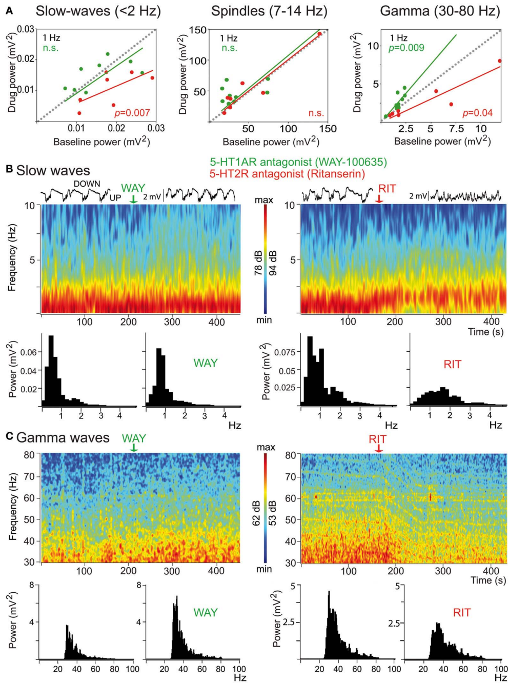
FIGURE 8 | Distinct modulation of cortical synchrony by 5-HT 1A and 5-HT 2A/2C receptors. (A) Effects of the 5-HT 1A antagonist WAY (green) and the 5-HT 2A/2C R antagonists ritanserin (RIT, red) on the baseline power (comparison of 30 s epochs before and after drug injection) of slow, spindle, and gamma oscillations. Note the opposing actions of the two drugs on the power of gamma oscillations. (B) Examples of the effects of WAY and RIT on the power of slow waves. Time-frequency
