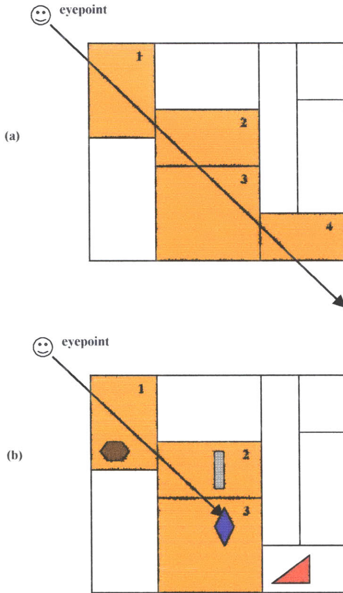
Figure 4.4.2.1 - Shooting a Ray Through a K-d Tree
