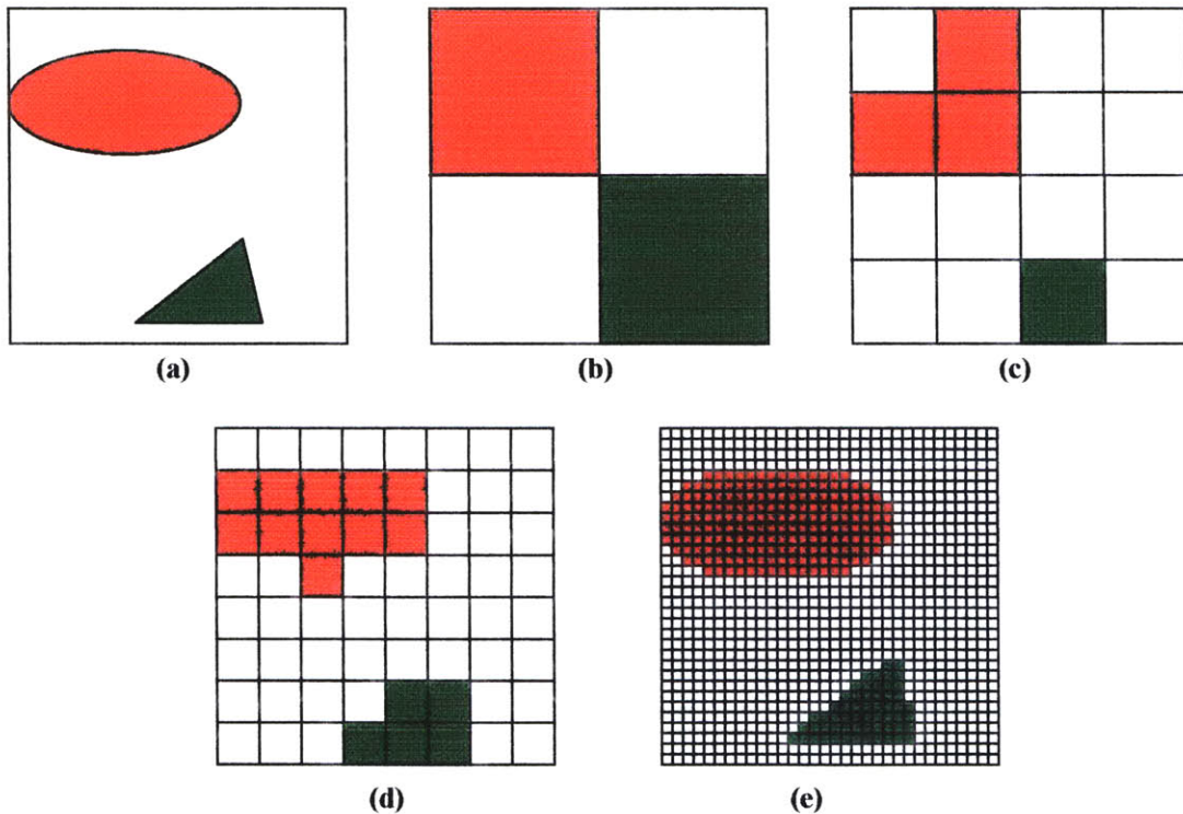
Figure 4.4.2.4 - Progressive Rendering An example of progressive rendering. (a) This is how the finished scene should look. (b), (c), (d) The first three resolutions of progressive rendering of the scene. (e) Several resolutions later, as the size of each block approaches one pixel. (continued on next page)
