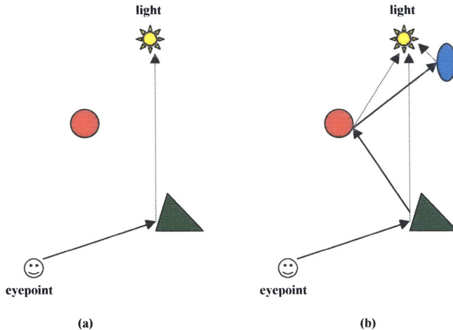
Figure 4.4.2.2 - Maximum Depth (a) Maximum depth equals one. (b) Maximum depth equals three. More detailed shading information can be obtained with greater depth values. At each intersection point, rays are fired from the point to light sources in the scene to get shading information from direct lighting. Reflection rays provide shading information from indirect lighting being reflected off of other objects. The dashed arrows indicate rays being fired directly to the light source from intersection points.
