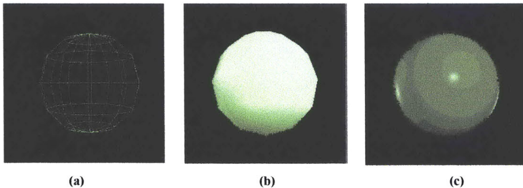
Figure 4.4.1.1 - Spheres (a) A wireframe sphere and (b) a solid sphere as rendered by JGL. (c) A sphere rendered by the ray tracer is shown for comparison.
