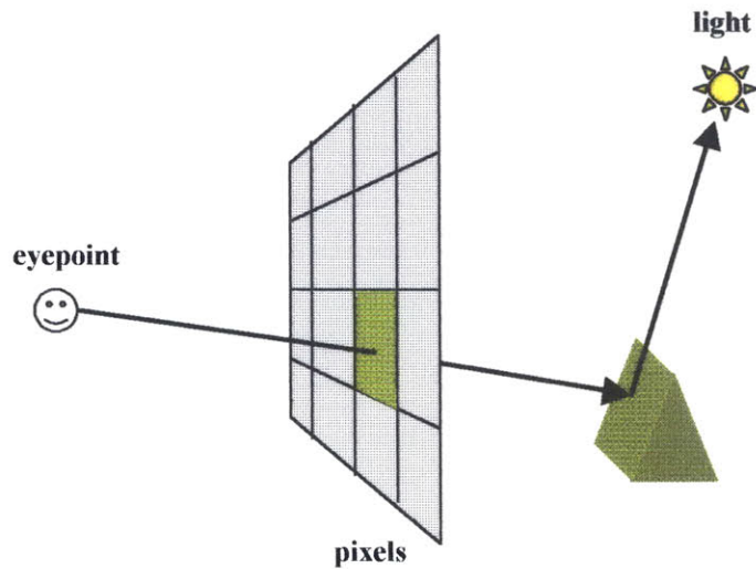
Figure 1.1 - Ray Tracing The ray tracing algorithm fires rays from the eyepoint through each pixel of the image to determine what object is visible through that pixel and the corresponding color to shade the pixel.
