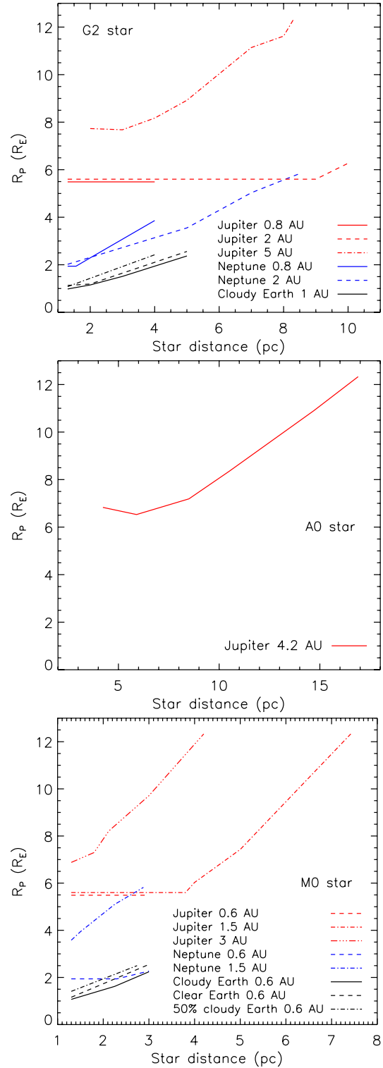
Fig. 20. Minimum radius of model planets for which characterization is possible (see text) for different star types: G2 (top), A0 (middle) and M0 (bottom). We slightly offset for clarity the curves of the 0.8-AU Jupiter (top) and 0.6-AU Jupiter (bottom). Note that for lack of space, we do not indicate the labels for all Earths in the top panel, but they are the same as those of the bottom panel except for the planet separation.
