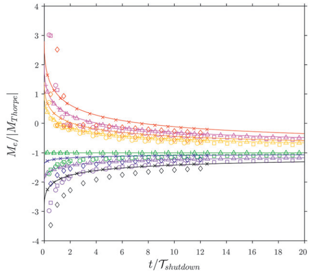
FIG. 5. Numerical and analytical solutions for the Ekman transport during buoyancy shutdown from all configurations, where U/|U_{\text{Thorpe}}| = -2.8 (black), -2 (purple), -1.4 (blue), -1 (green), 1 (yellow), 1.4 (orange), 2 (magenta), and 2.8 (red). The symbols are defined in Fig. 4 for simulations with constant and Richardson number–dependent mixing coefficients. Time is nondimensionalized by (10) from the constant diffusivities.
