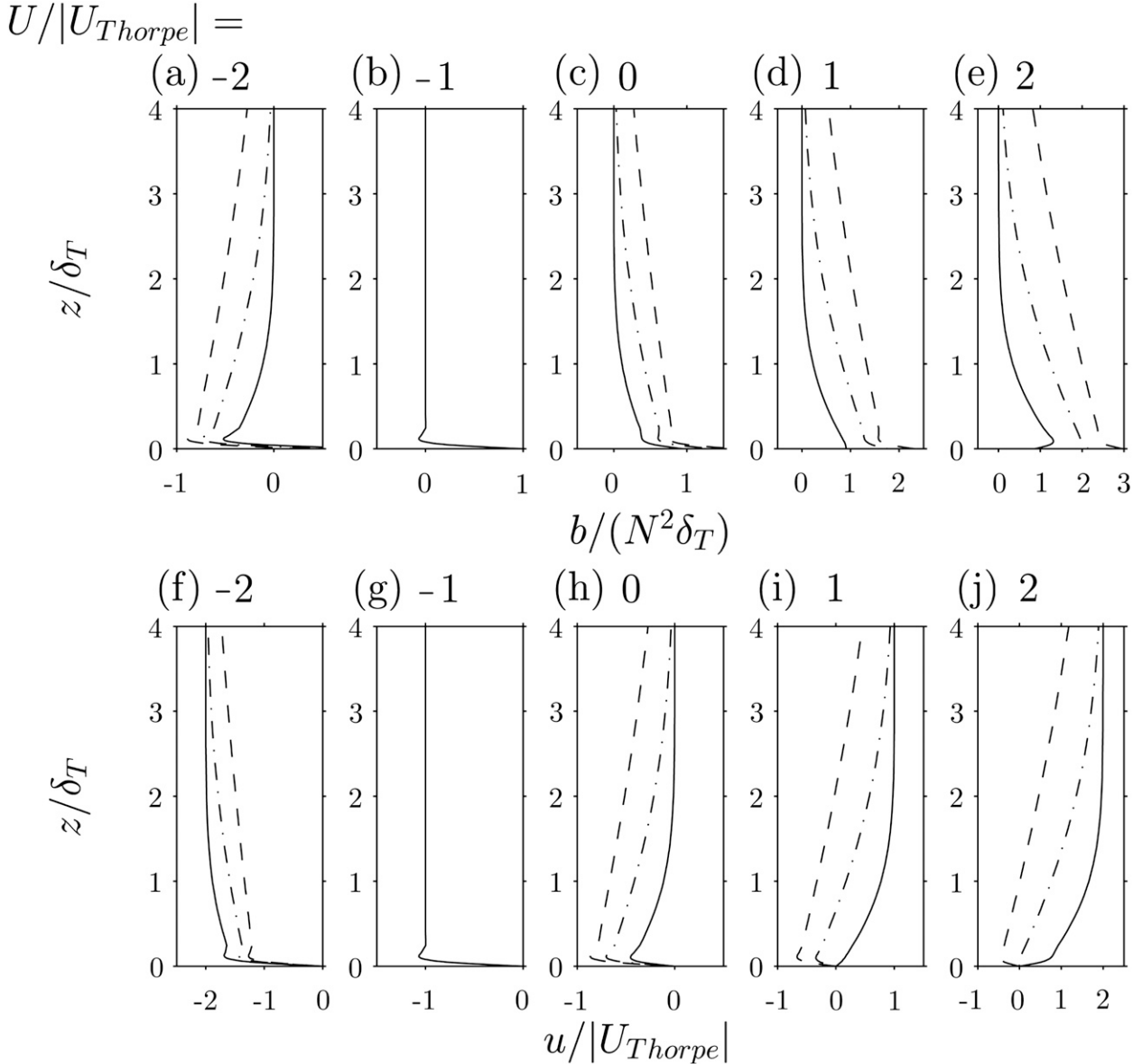
FIG. 2. (a)–(e) Analytical solution for the buoyancy and (f)–(j) the along-isobath flow evaluated at t/T = 1 (solid), 5 (dashed–dotted), and 20 (dashed), with S = 0.05 . The Ekman layer thickness is \delta_e/\delta_T = 0.05 in this example. Time is nondimensionalized by the buoyancy generation and shutdown time scale T = \sigma^{-1}S^{-2}f^{-1} , (16) and (10).
