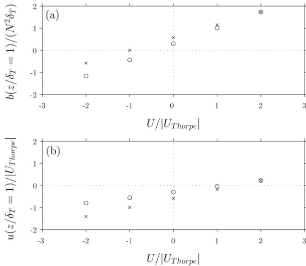
FIG. 7. The (a) buoyancy anomaly and (b) along-isobath flow at z/\delta_r = 1 at 800 inertial periods from configuration 1: high mixing and low N^2 . The values are from constant (crisscrosses) or Richardson number–dependent mixing (circles).
