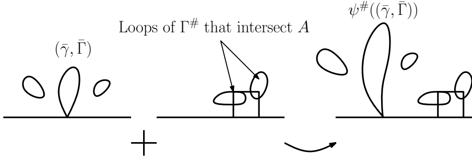
Figure 17: The measure \mu_A^\# (sketch)
