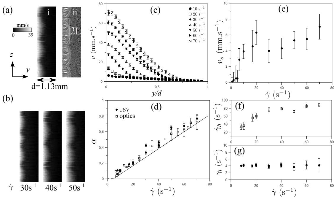
FIG. 3: (a) Comparison between (i) velocity measurements and (ii) optical visualizations of the shear-banding flow of a solution of [\text{CTAB}]=0.3 \text{ M} , [\text{NaNO}_3]=0.4 \text{ M} , T=28^\circ\text{C} , \Lambda \simeq 0.08 , at \dot{\gamma} = 40 \text{ s}^{-1} . (i) USV measurements. Each horizontal line is a velocity profile v_\theta(y) at a given location z along the vorticity axis, with the velocity encoded as a grey level between the zero velocity at the fixed outer cylinder (right) and v_w=39 \text{ mm/s} , the velocity at the moving inner cylinder (left). Measurements along z were done every 100 \mu\text{m} , which is above the vertical resolution of the transducer ( 65 \mu\text{m} ). The time interval between each velocity profile is between 0.5 and 1 \text{ s} depending on the applied shear rate. (ii) Overlay of two optical visualization techniques showing the secondary vortex flow in the high shear rate band. The first technique, with the red laser, gives the strong turbidity contrast between the bands. The second technique, with white light, allows for the observation of the vortices. (b) Velocity profiles along the vorticity axis for \dot{\gamma} = 30, 40, 50 \text{ s}^{-1} . The velocity is encoded as a grey level between 0 and v_w(\dot{\gamma}) . (c) Time averaged velocity profiles v_x(y) at a given location z for various shear rates. (d) Proportion of the high shear rate band as a function of \dot{\gamma} measured from the optical or USV protocols. (e) Slip velocity at the inner cylinder as a function of \dot{\gamma} . (f) Local shear rate in the high shear rate band ( \dot{\gamma}_h ) as a function of \dot{\gamma} . (g) Local shear rate in the low shear rate band ( \dot{\gamma}_l ) as a function of \dot{\gamma} .
