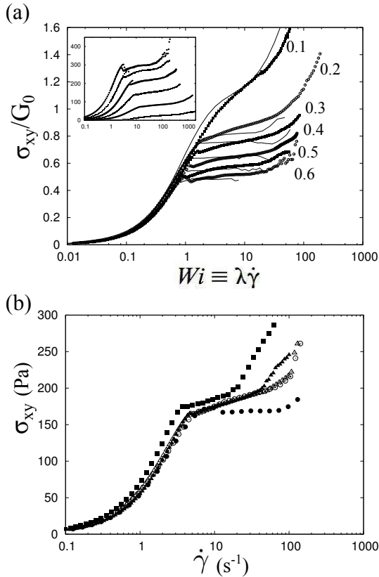
FIG. 2: (a) Experimental flow curves obtained for various concentrations of [CTAB]=0.1, 0.2, 0.3, 0.4, 0.5 and 0.6 M at a constant salt concentration [NaNO 3 ]=0.3 M and constant temperature T=30^\circ\text{C} . The flow curves were obtained by increasing the imposed shear rate. The shear stress is in units of G_0 and the shear rate is made dimensionless by using the Weissenberg number Wi \equiv \lambda\dot{\gamma} . The flow curves with the symbols (■ and ○) were obtained on a TC device with d = 1.13 mm and R_i = 13.33 mm, with two minutes spent on each data point. The continuous lines are the corresponding flow curves obtained in cone-and-plate geometry (2 min/point). Inset: TC flow curves in dimensional form ( \sigma_{xy} vs \dot{\gamma} ), stacked from top to bottom in between [CTAB]=0.6 M and [CTAB]=0.1 M. For each system, two runs are plotted, one with a sampling time of 2 min/point (corresponding to the dimensionless data) and one with only 5 s/point. (b) Experimental flow curves for a system with [CTAB]=0.3 M, [NaNO 3 ]=0.4 M and T=28^\circ\text{C} . The flow curves are obtained in different shearing geometries: cone-and-plate (●) and TC with \Lambda = 0.04 (○), 0.08 (△), 0.2 (▲) and 0.9 (■); 2 min/point.
