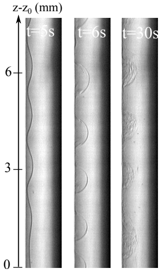
FIG. 10: Three snapshots of the gap of a solution of [\text{CTAB}] = 0.55 \text{ M} in \text{D}_2\text{O} (20 wt %) at T = 37.5^\circ\text{C} , in a TC cell with \Lambda = 0.08 . The gap is illuminated by white light (the illumination is made non-homogeneous in the gap in order to increase the contrast between the high and low shear bands). The three pictures are taken a few instants after the onset of a start-up flow with \dot{\gamma} = 50 \text{ s}^{-1} . The last picture ( t = 30 \text{ s} after the onset of shear) is representative of the asymptotic state.
