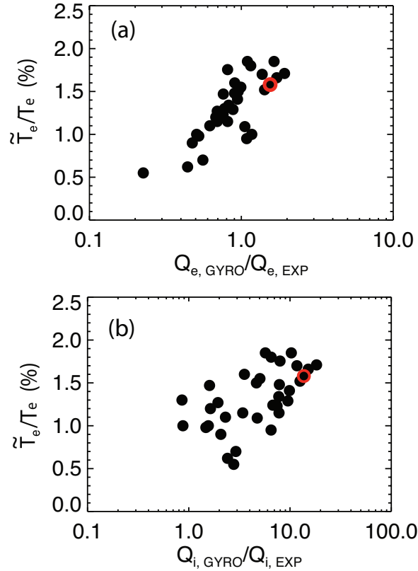
Figure 10. (Colour online) Fluctuation level plotted against (a) Q_e^{GYRO}/Q_e^{EXP} and (b) Q_i^{GYRO}/Q_i^{EXP} from series of L-mode simulations. The open red circle corresponds to the local simulation from Section 4 (b)
