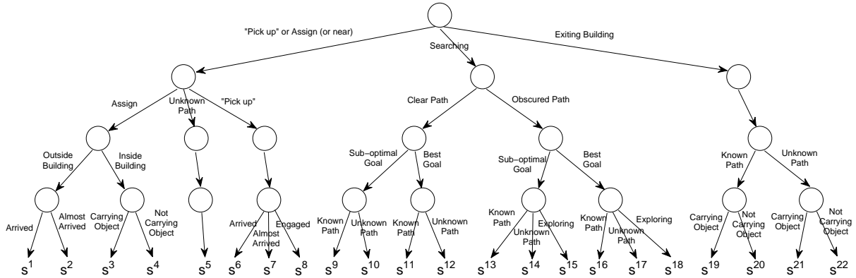
Figure 3. The decision tree used to define a UV's state in the user study.
