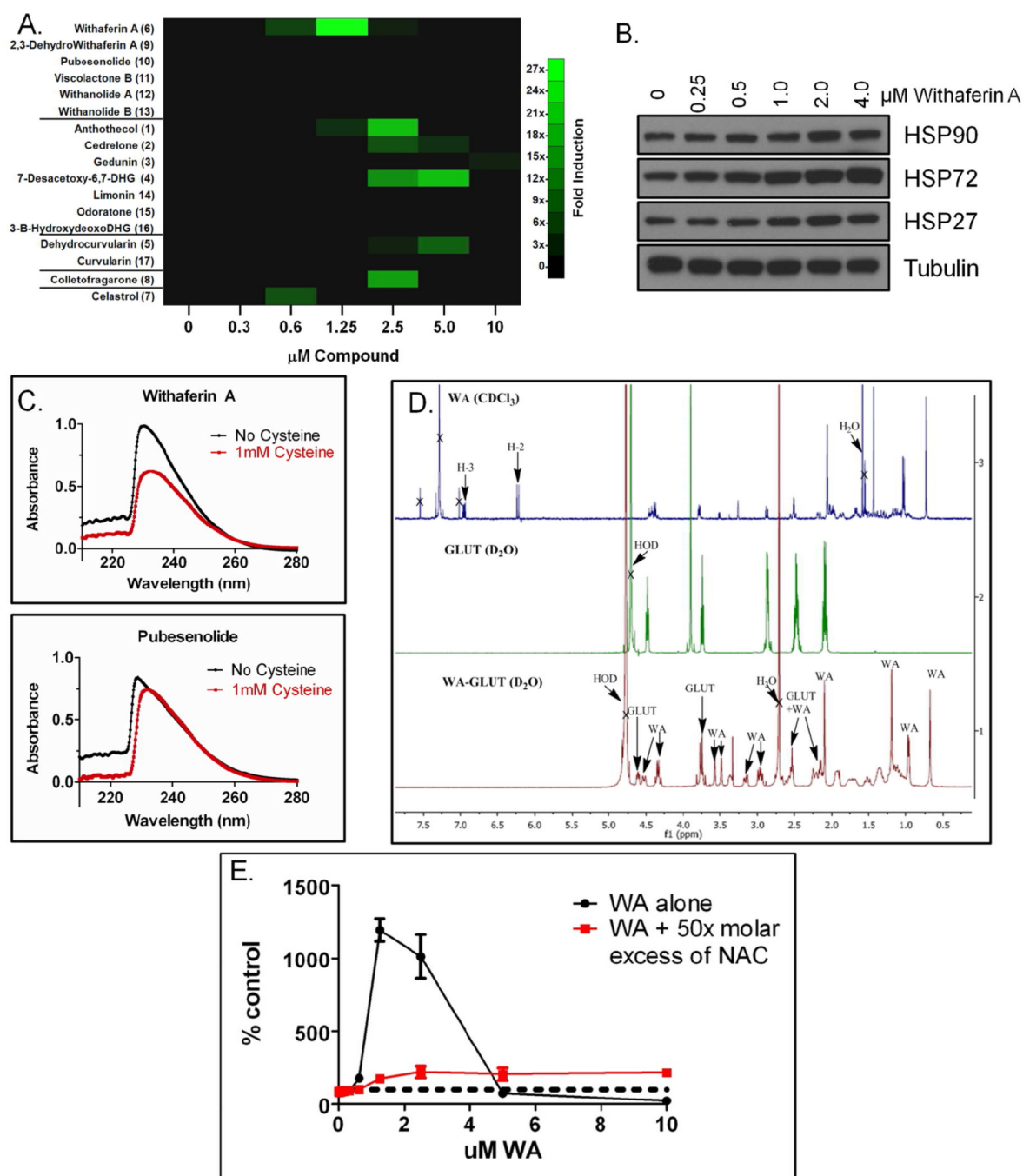
Figure 3. Thioreactive natural products induce a heat-shock response. a) Heat map of HSE-eGFP induction compared to vehicle only. Determinations were in triplicate. b) Immunoblot analysis of LN428 following treatment with indicated amounts of WA (6) for 16 hours. c) UV absorption spectra of WA (6) and pubesensolide (10) with or without Lcysteine. d) NMR spectra of WA (6) with or without glutathione. e) Heat-shock reporter activation by WA alone and in the presence of a 50x molar excess of n-acetylcysteine (NAC). Dashed line at 100% indicates baseline level of reporter signal. Decrease below 100% reflects cytotoxicity.
