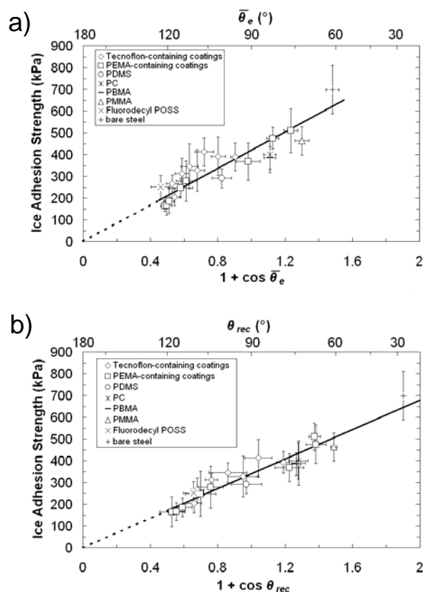
Figure 4. Average shear strengths of ice adhesion measured at -10 °C for bare steel and 21 different coatings plotted against water contact angle parameters that scale with (a) the equilibrium work of adhesion for liquid water (see Equation (2)) and (b) the practical work of adhesion for liquid water (see Equation (3)). The straight lines are the linear best fits that pass through each origin, with the solid portions of the lines encompassing the measured data and the dashed portions representing the extrapolation to the origin. The linear fit for (b) ( \tau_{ice} = (340 \pm 40 \text{ kPa})(1 + \cos \theta_{rec}) , R^2 = 0.92 ) is significantly better than that for (a) ( R^2 = 0.80 ).
