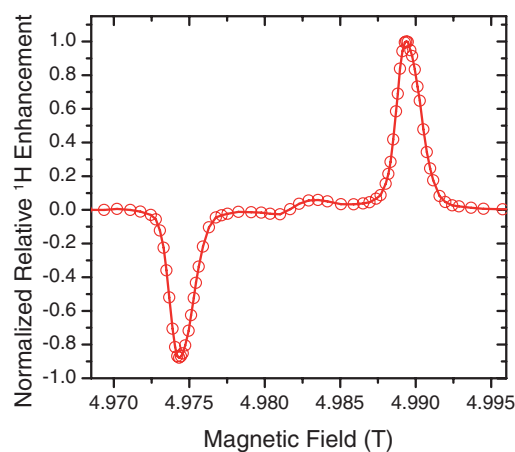
FIG. 3. 140 GHz DNP enhancement field profile for a 40 mM solution of trityl (OX063) in a mixture of 60:30:10 vol.-% d_8 -glycerol/ D_2O/H_2O recorded with a gyrotron microwave output power of 8 W at 85 K and 5 kHz MAS. Data points were obtained by recording the amplitude of the enhanced ^1H Bloch decay FID.
