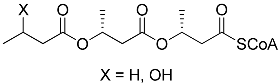
Figure 1. Structure of (HB) 3 CoA and sTCOA. Primers for in vitro production of PHB by PhaC Ec . (HB) 3 CoA, X=OH. sTCOA, X=H.
