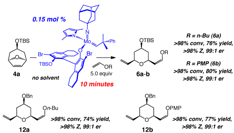
Scheme 1. Highly Efficient Mo-Catalyzed Z-Selective EROCM Reactions a
