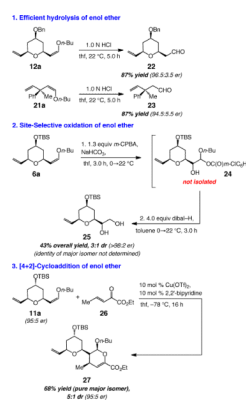
Scheme 2. Representative Functionalization Procedures with Enantiomerically Enriched Enol Ethers Obtained through Mo-Catalyzed ROCM reactions
