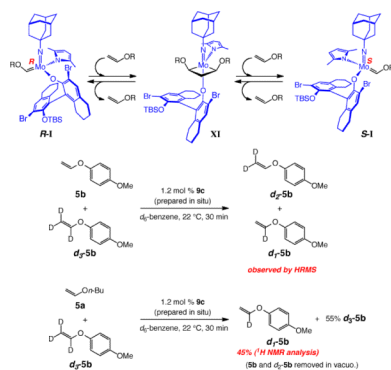
Scheme 5. Interconversion of Diastereomeric Mo Complexes through Non-Productive Olefin Metathesis a
