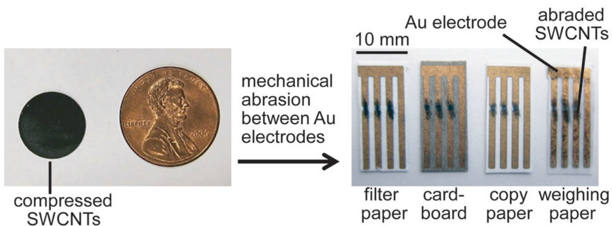
Figure 1. Fabrication of sensors on various types of paper by mechanical abrasion of compressed SWCNTs.
