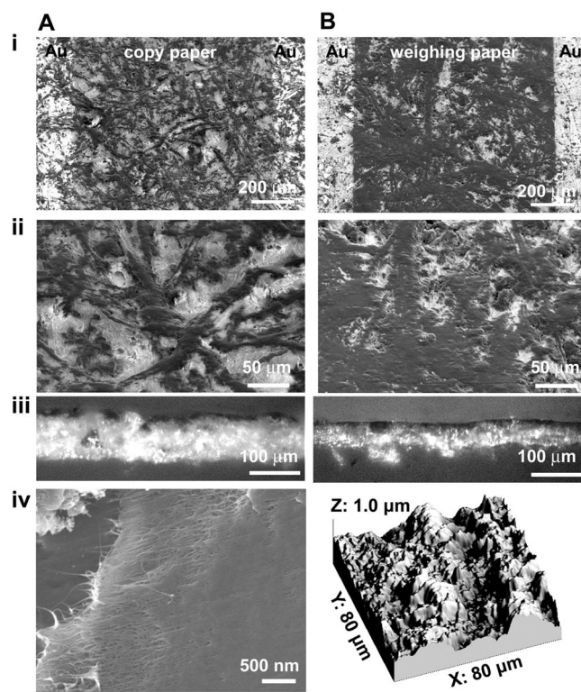
Figure 2. Imaging and characterization of sensors fabricated by mechanical abrasion of pristine SWCNTs on copy paper (A) and weighing paper (B). i–ii) Scanning Electron Microscopy (SEM) images of SWCNTs abraded on copy paper (A) and weighing paper (B). iii) Optical micrographs of cross-sections of copy paper (A) and weighing paper (B) containing SWCNTs deposited by abrasion. iv) High magnification SEM image of SWCNTs abraded on the surface of copy paper (A), and Atomic Force Microscopy image of SWCNTs abraded on the surface of weighing paper (B).
