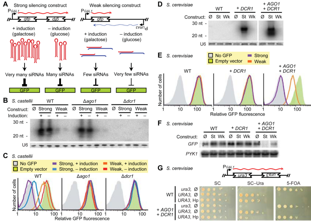
Fig. 4. Engineering RNAi in S. castellii and S. cerevisiae . (A) Schematic for silencing of a GFP reporter. The strong silencing construct included inverted repeats of a gfp fragment and was designed to produce a hairpin transcript (38). The weak silencing construct contained one copy of the fragment, which is transcribed convergently to produce dsRNA. (B) RNA blot probing for siRNAs antisense to GFP , using total RNA from the indicated S. castellii strains with integrated empty vector ( \emptyset ) or silencing construct (strong or weak), either induced with galactose (+) or uninduced (-). The blot was reprobbed for U6 small nuclear RNA. (C) FACS histograms showing GFP fluorescence in the indicated S. castellii strains expressing the indicated silencing constructs. (D) RNA blot probing for siRNAs antisense to GFP in S. cerevisiae strains expressing either no S. castellii genes (WT) or the indicated integrated S. castellii genes, and either the strong (St), the weak (Wk), or no ( \emptyset ) silencing construct. The blot was reprobbed for U6 small nuclear RNA. (E) FACS histograms showing GFP fluorescence in the indicated S. cerevisiae strains expressing the indicated silencing constructs. All strains were induced; silencing from uninduced constructs was similar for the strong construct and undetectable for the weak construct (fig. S9). (F) RNA blot probing for GFP mRNA in the indicated S. cerevisiae strains expressing the indicated silencing constructs. The blot was reprobbed for PYK1 mRNA as a loading control. (G) Silencing an endogenous gene. S. cerevisiae strains containing non-functional and functional URA3 genes ( ura3 and URA3 , respectively) and expressing the indicated S. castellii genes and either the diagrammed hairpin construct (Hp) or no silencing construct ( \emptyset ) were tested for Ura3p expression by plating serial dilutions on complete media (SC), media lacking uracil (SC-Ura), and media containing 5-FOA (to which cells producing Ura3p are sensitive).
