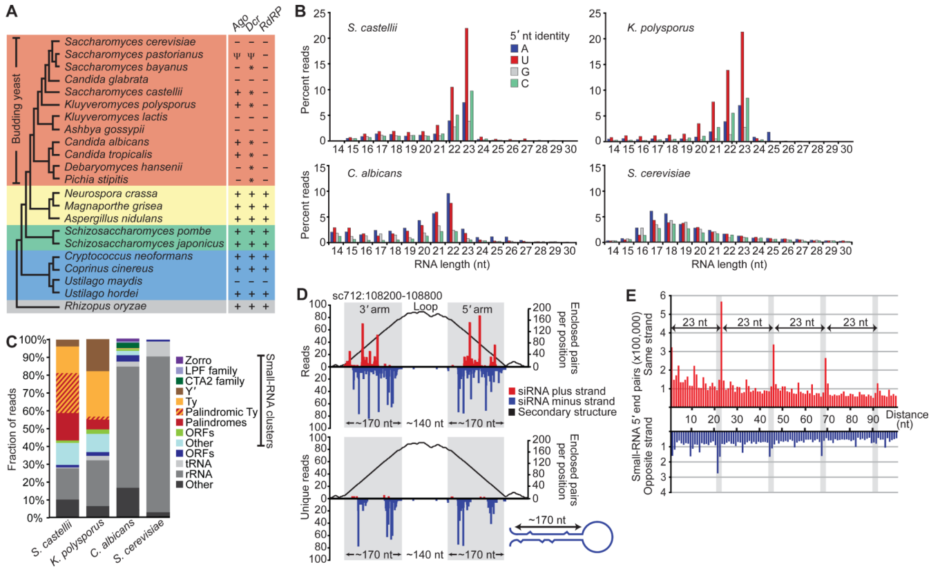
Fig. 1. Endogenous siRNAs in budding yeasts. (A) Cladogram showing Basidiomycota (blue), Zygomycota (grey) and Ascomycota, subdivided into Saccharomycotina (budding yeasts, orange), Pezizomycotina (yellow) and Taphrinomycotina (green) (35, 36). The presence of canonical RNAi genes is indicated (+) (4, 5) and references therein. All genomes had a RNT1 ortholog, and several others had a second RNaseIII domain-containing gene (*), which has Dicer activity in S. castellii . Pseudogenes are indicated (ψ). S. bayanus , which had a Dicer but not an Argonaute gene, appeared to lack siRNAs (fig. S1). (B) Length distribution of genome-matching sequencing reads representing small RNAs with the indicated 5' nucleotide. Reads matching rRNA and tRNA are excluded. (C) Classification of loci to which 21–23-mers map, considering those that map to clusters in a pattern suggestive of siRNAs separately from those that do not. (D) A palindromic region generating siRNAs in S. castellii . 5' termini of 22–23-mers were mapped to the genome, and counts (normalized to the number of genomic matches) are plotted for the plus and minus genomic strands. The top graph considers all reads; the bottom considers those matching the genome at only one locus. The predicted structure of the (–)-strand transcript is represented as a mountain plot (37). (E) Distribution of the genomic intervals separating the 5' termini of sequenced 23-mers from S. castellii . Plotted is the frequency of each interval, when considering all pairs of reads less than 100 nt apart (excluding reads matching rRNA and tRNA).
