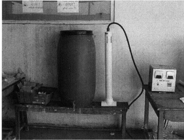
Figure 3.1: Sodium Hypochlorite Generator in Kathmandu, Nepal (Morganti, 2002)
