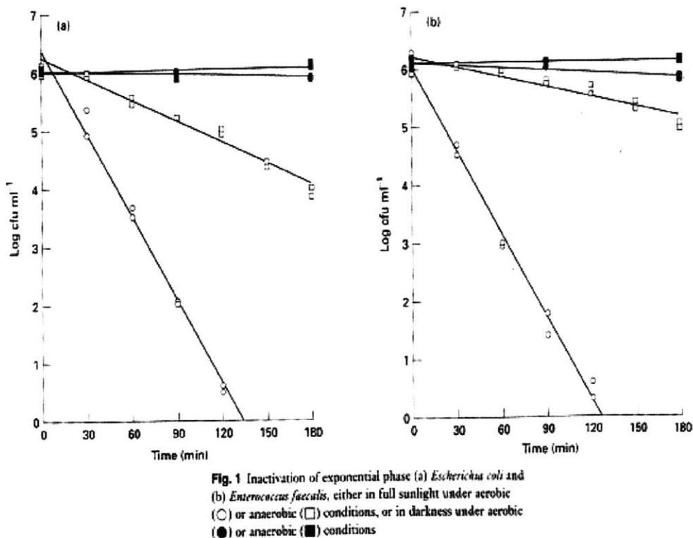
Figure 2-5. Aerobic vs. Anaerobic Microbial Inactivation (Reed, 1997).
