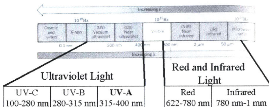
Figure 2-2. Important Components of the Electromagnetic Spectrum (Solomon, 1996)
